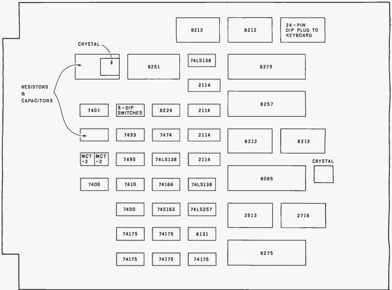
Figure 3: Diagram of the parts layout on the component side of the main circuit board of the video terminal. A type 4350 Vector wire-wrap board was used.
