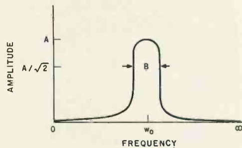
TYPICAL BANDPASS FILTER RESPONSE CURVE
