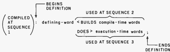
Figure 4: The structure of the source definition of a defining word. These source lines create a defining word for a new family (sequence 1). Execution of the defining word (sequence 2) <BUILDS a dictionary definition for a new family member. The contents of that definition is constructed by the compile-time words. Executing any family member (sequence 3) DOES> (ie: executes) the execution-time words.
