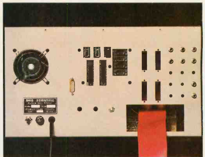
Photo 2: Rear panel of an Ohio Scientific C8P computer, showing connections from the CA-15 universal telephone interface to outside components. The board connects to a CBT-type data coupler through the DB-15 connector (the small gold-colored connector in the center of the back panel). Other connections are made through the six phono jacks in the upper right-hand corner of the back panel. The jacks, listed in row order from left to right, are: cassette-recorder on/off control, phone-line monitor output, Votrax output (if used), cassette-player on/off control, cassette-player input, and auxiliary input.
