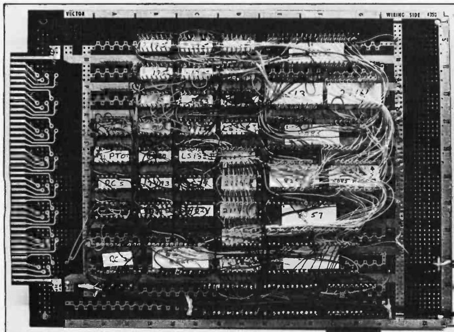
Photo 2: The bottom or wired side of the video terminal board.
