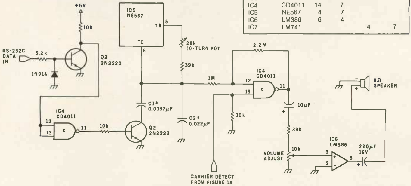
Figure 1b: Modulator section of the modem circuit in schematic form. The tone frequency for a mark (1270 Hz) is set up by choosing the proper values for capacitor C2 and adjusting the 20 k-ohm potentiometer. When transistor Q2 gates capacitor C1 in parallel with C2, the oscillator frequency changes to 1070 Hz.
