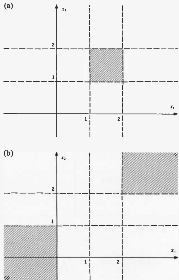
Figure 1: Consistent and inconsistent systems of linear inequalities. The shaded area in figure 1a represents the solution set of the four inequalities, x_1 \geq 1 , x_1 \leq 2 , x_2 \geq 1 , x_2 \leq 2 . Since points exist that satisfy all four inequalities, the system is said to be consistent. The system shown in figure 1b is inconsistent. The lower shaded area is given by the equations x_1 \leq 1 and x_2 \leq 1 ; the upper shaded area is given by x_1 \geq 2 and x_2 \geq 2 . No point satisfies all four inequalities simultaneously.
