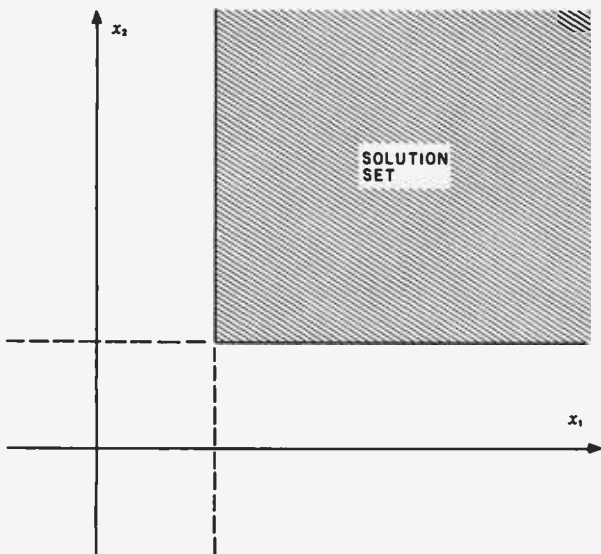
Figure 2: A set of linear inequalities. The shaded area represents the solution set of the two inequalities, x_1 \geq 1 and x_2 \geq 1 . Figure 3 shows how Khachiyan's algorithm solves this system of linear inequalities.
