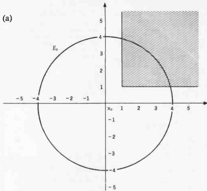
Figure 3: A graphic example of Khachiyan's algorithm. The Khachiyan algorithm (described here for a two-dimensional problem) begins with a circle centered at the origin with a radius of a given size such that the circle is guaranteed to contain the solution points, if they exist. Successive iterations of Khachiyan's algorithm produce ellipses of smaller area that still contain the solution points. Here, the initial circle E_0 is shown in figure 3a. Ellipse E_1 is then computed from E_0 , as shown in figure 3b, and ellipse E_2 is computed from E_1 , as shown in figure 3c. In the last two figures, the current ellipse is shown in black, and the previous ellipse is shown in gray. The shaded area in all three figures describes the inequalities' solution set.
