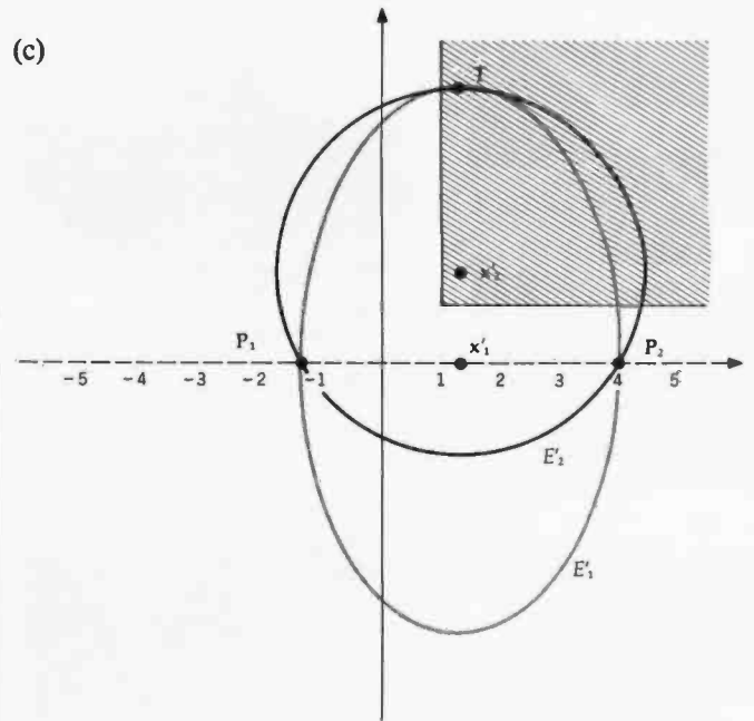
Figure 3: A graphic example of Khachiyan's algorithm. The Khachiyan algorithm (described here for a two-dimensional problem) begins with a circle centered at the origin with a radius of a given size such that the circle is guaranteed to contain the solution points, if they exist. Successive iterations of Khachiyan's algorithm produce ellipses of smaller area that still contain the solution points. Here, the initial circle E_0 is shown in figure 3a. Ellipse E_1 is then computed from E_0 , as shown in figure 3b, and ellipse E_2 is computed from E_1 , as shown in figure 3c. In the last two figures, the current ellipse is shown in black, and the previous ellipse is shown in gray. The shaded area in all three figures describes the inequalities' solution set.
