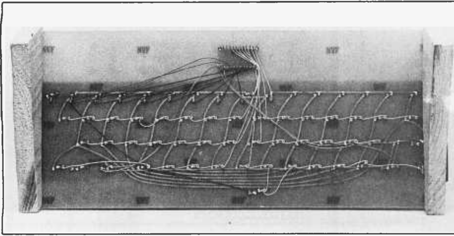
Photo 4: The etch side of the keyboard circuit board, showing the jumper connections made necessary by use of the single-sided board.
