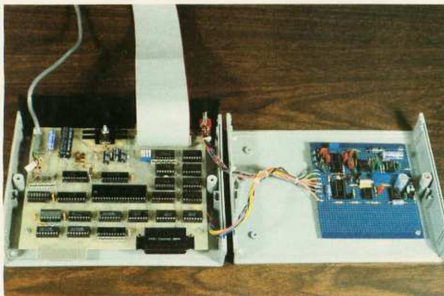
Photo 1: The prototype modem circuit of figure 1 was assembled on the blue perforated circuit board as shown. It was then installed under the top cover of a COMM-80 I/O-expansion unit, shown at left. The COMM-80 was described in the June Circuit Cellar. (See "I/O Expansion for the TRS-80, Part 2: Serial Ports," June 1980 BYTE, page 42.) The COMM-80 and this modem are sufficient to turn a Radio Shack TRS-80, or a computer that uses a similar bidirectional bus, into a timesharing terminal. The modem can be used on any computer.
