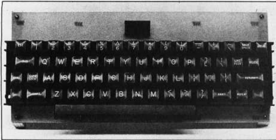
Photo 3: The sixty-three-key Jameco keyboard mounted on its printed-circuit board and installed on support blocks.
