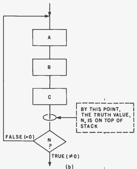
Figure 4: An explanation of the BEGIN ... UNTIL construct. As shown in figure 4a, the body of the loop (shaded) is repeated only if the value on top of the stack when the word UNTIL is reached is false. Figure 4b gives the equivalent construct in conventional flowchart notation.
