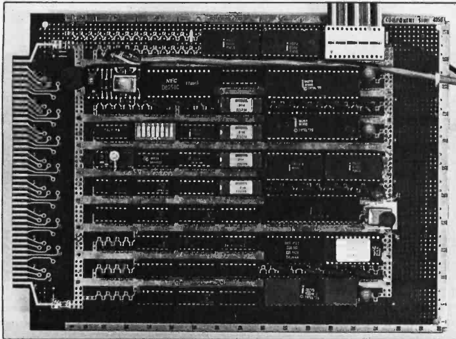
Photo 1: The complete video terminal circuitry constructed on a wire-wrap board. The component side is shown.
