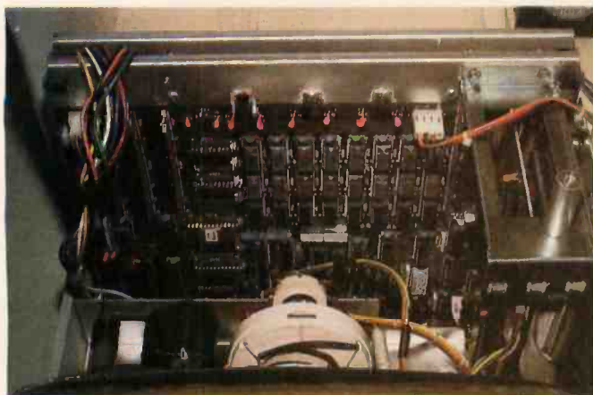
Photo 2: Interior of the Heath H-89 computer.
