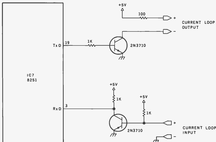
Figure 2: Schematic diagram of the temporary interface for connecting the checkout terminal to the new terminal for debugging.
