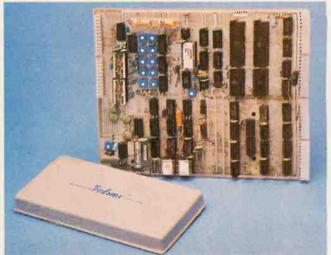
Photo 1: The CA-15 universal telephone interface board, shown with its optional Votrax voice synthesis module.
