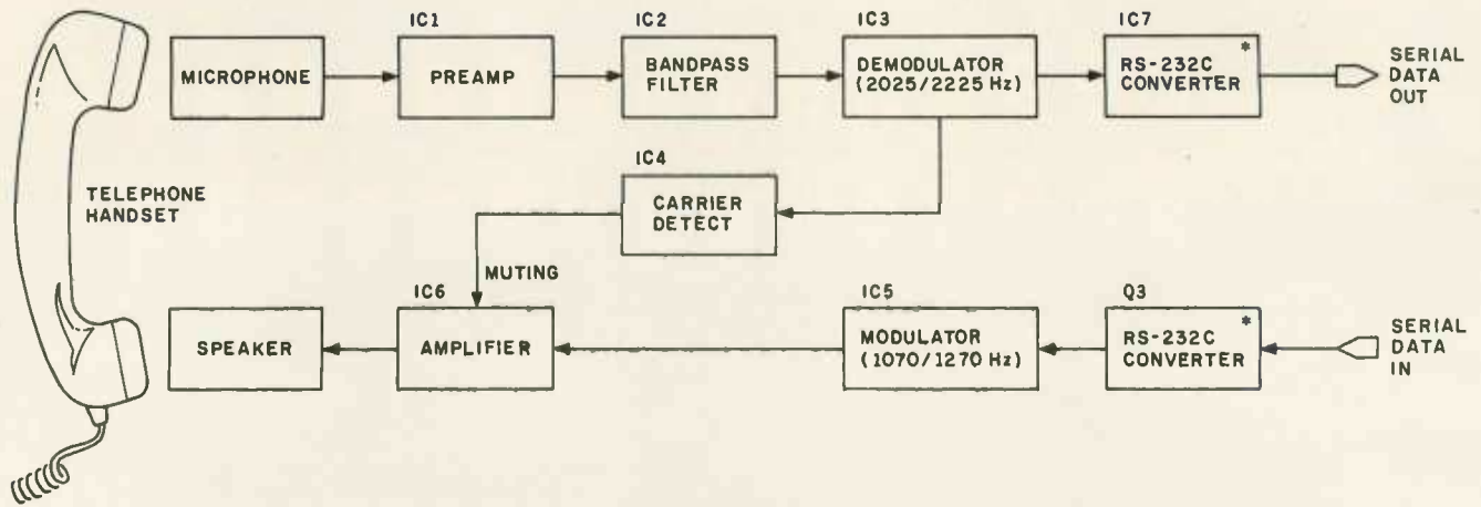
Figure 2: Block diagram of the originate-only modem presented in this article. The blocks marked with asterisks (*) indicate the components that provide RS-232C compatibility; these may be left out of the circuit if RS-232 communication is not needed.
