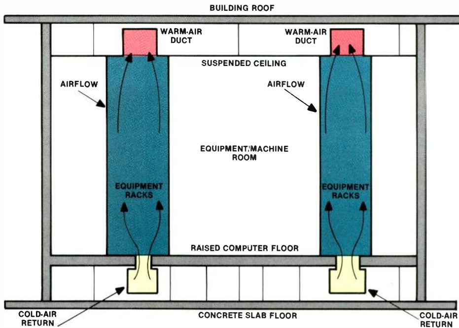
Figure 3. Air-conditioning airflow for cooling equipment racks in the control rooms of studios 2 and 4.
