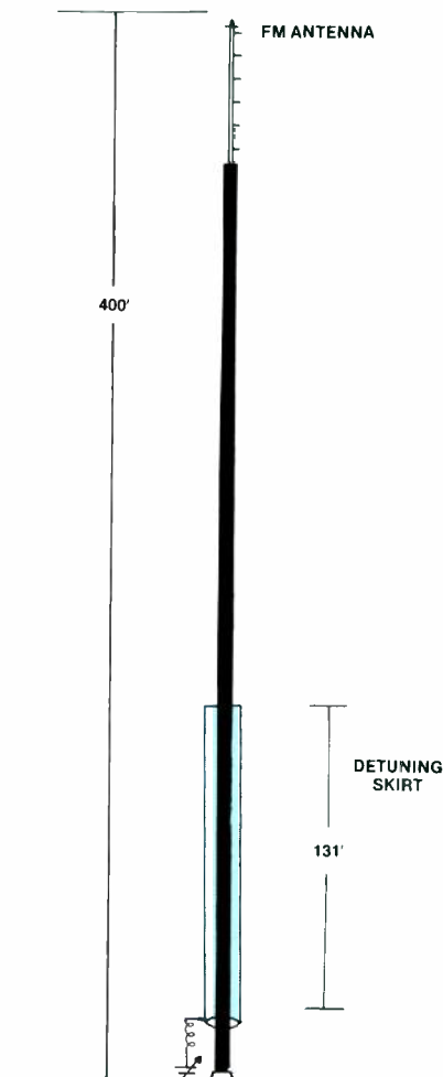
Figure 1. Detuning skirt for a tall FM tower located close to an AM radiator.
