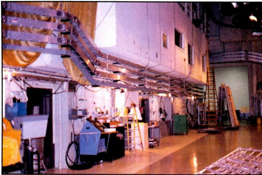
The Studio 4 sound stage floor showing the cable ladder tracks. A 4-layer cabling configuration is used. The trays (from top to bottom) carry low-level microphone lines; video and high-level audio; camera and communications; and regulated ac (technical) power.
