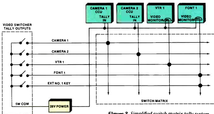
Figure 3. Simplified switch-matrix tally system.
