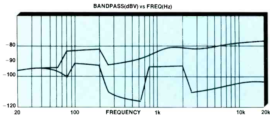
Figure 5. Noise floor sweep. Upper curve shows better than -75\text{dBV} noise with the output control fully open. Lower curve shows better than -90\text{dBV} noise with the output control fully closed.
