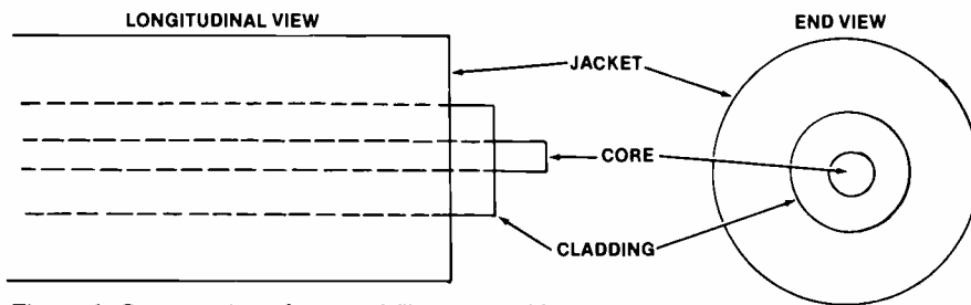
Figure 1. Cutaway view of a typical fiber-optic cable.
