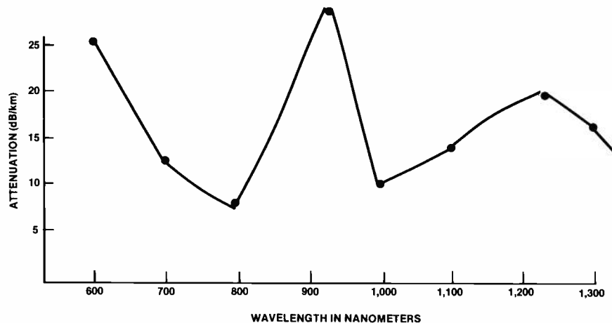
Figure 6. Typical attenuation curve of polymer-clad, glass fiber. Note the ideal operating windows at about 750nm to 850nm and 1,000nm upward.
