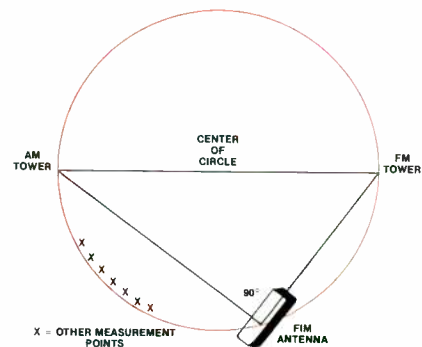
Figure 2. Measuring parasitic radiation with a field-intensity meter.
