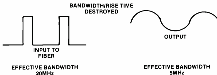
Figure 4. Effective bandwidth limitations created by modal dispersion.
