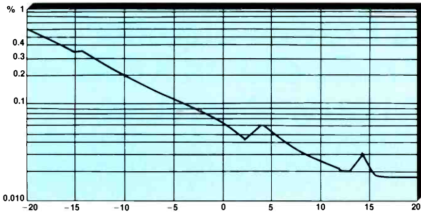
Figure 4. IMD distortion measured from -20dBm - +20dBm. The output shows less than 0.5% IMD for levels above -17dBm.
