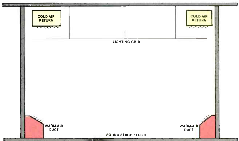
Figure 2. HVAC system layout for the sound stage of Studio 2.
