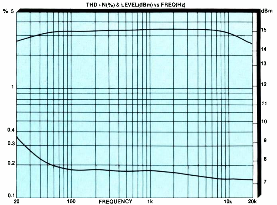
Figure 3. Line input frequency response (top curve). The lower curve shows the THD through the line input with 40dB of gain.
