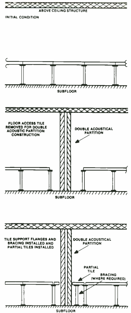
Figure 2. The existing computer-access flooring had to be specially modified to permit the construction of double acoustical partitions.
