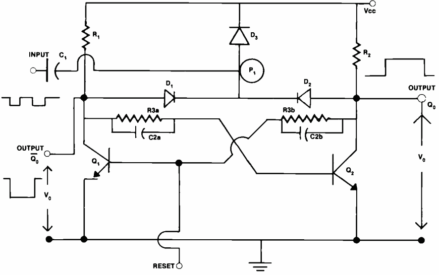
Figure 2. Bi-stable multivibrator typically used as a binary counter, by dividing the input frequency by 2.
