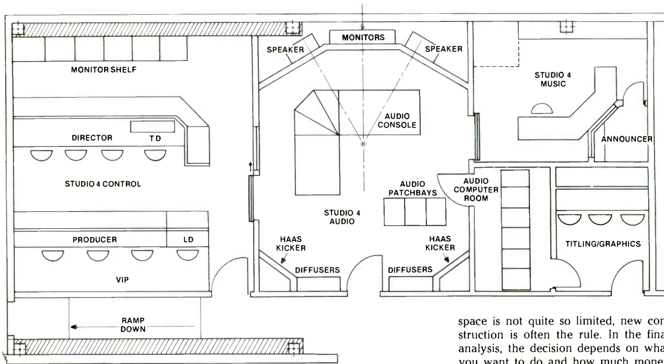
Figure 1. Basic floor plan for the control room area of Studio 4 at NBC's Burbank facility.
