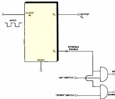
Figure 1. Logic symbol for a bi-stable flip-flop used in a transmitter remote-control circuit.
