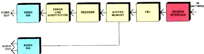
Figure 6. Block diagram of a typical video codec, used to convert TV signals from analog to digital, or digital to analog.
