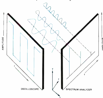
Figure 1. A comparison of oscilloscope (y-t) and spectrum analyzer (y-f) displays. A square wave consists of a fundamental and odd harmonics. Amplitudes of the harmonics are the reciprocal of the harmonic number.
