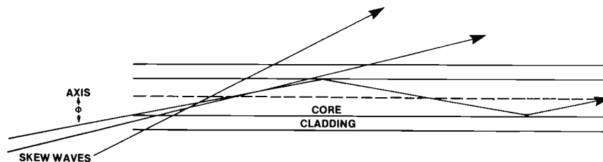
Figure 5. The acceptance angle of a fiber ( NA = \sin\theta ).
