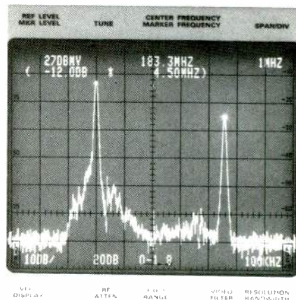
Figure 2. A spectrum analyzer display shows TV channel 8 visual and aural carriers. Photo courtesy of Tektronix.
