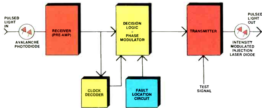
Figure 5. Functional diagram of a typical fiber-optic repeater.
