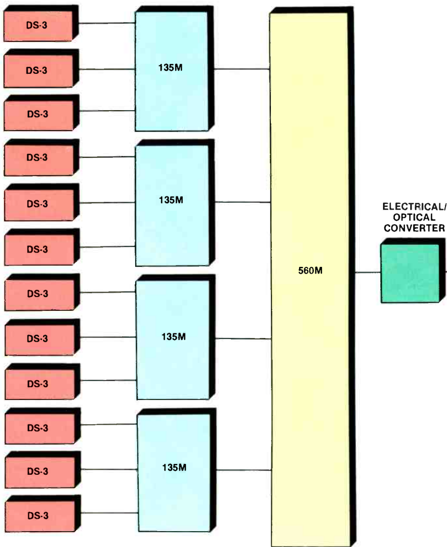
Figure 4. Block diagram of terminals located at the point-of-presence (POP) in each city.
