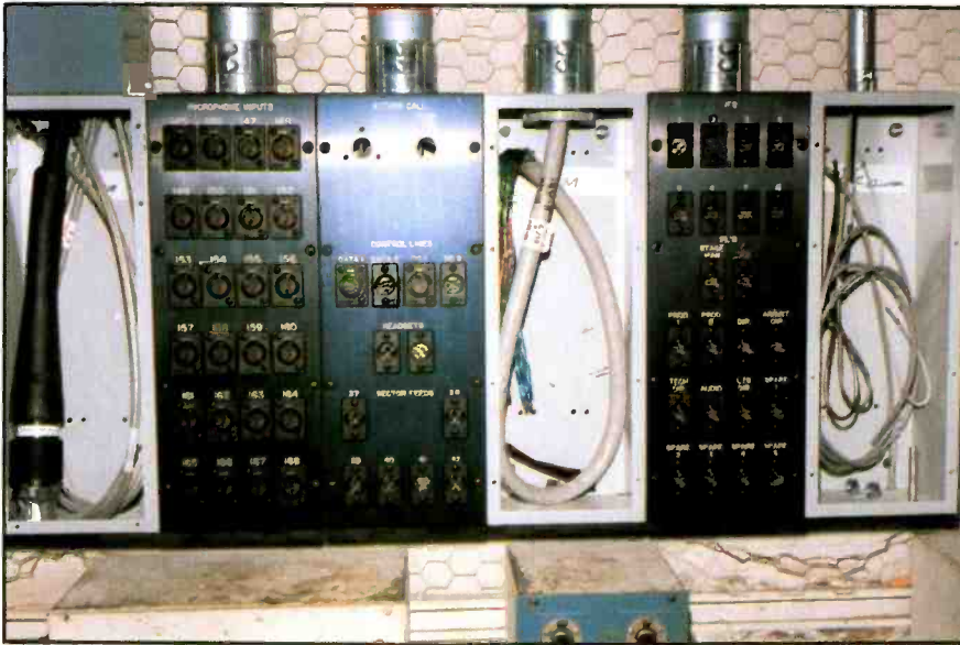
One of the eight drops installed on each sound stage floor during construction. The panels (left to right) provide connection points for camera and video tie trunks (unfinished panel); microphone inputs; actors' call lines; headsets/sector feeds (unfinished); PA lines; and IFB/com-munications (unfinished).
