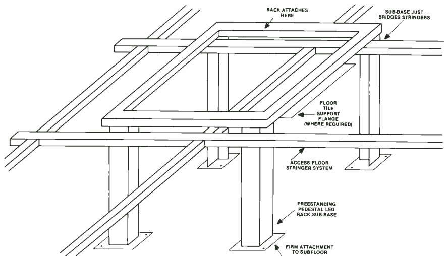
Figure 3. Special rack supports attach directly to the subfloor, keeping the racks independent of the computer-access flooring.
