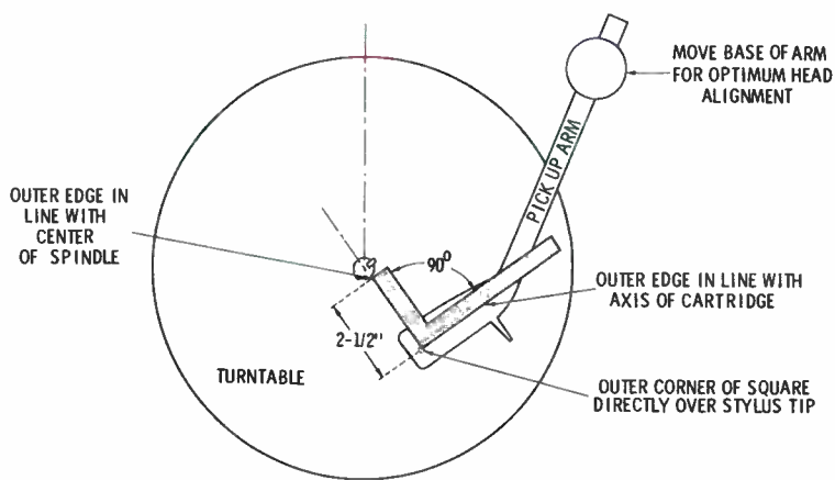
Fig. 1. Proper arm orientation is important in the reduction of record wear.
