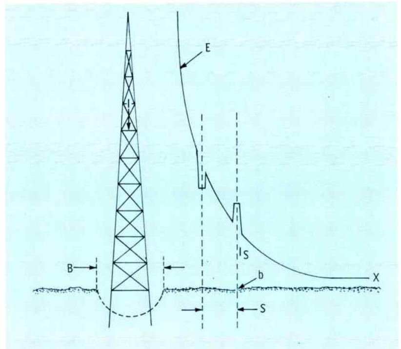
Fig. 2. The potential at the surface of the earth near an electrode containing lightning current. Note that the potential decreases as the distance from the tower is increased.
