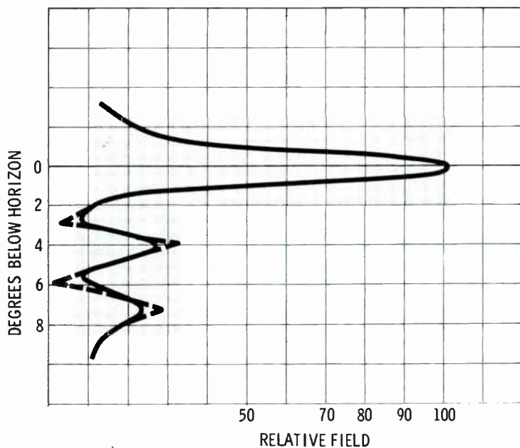
Fig. 4. Vertical pattern of horizontally polarized, very directional antenna.
