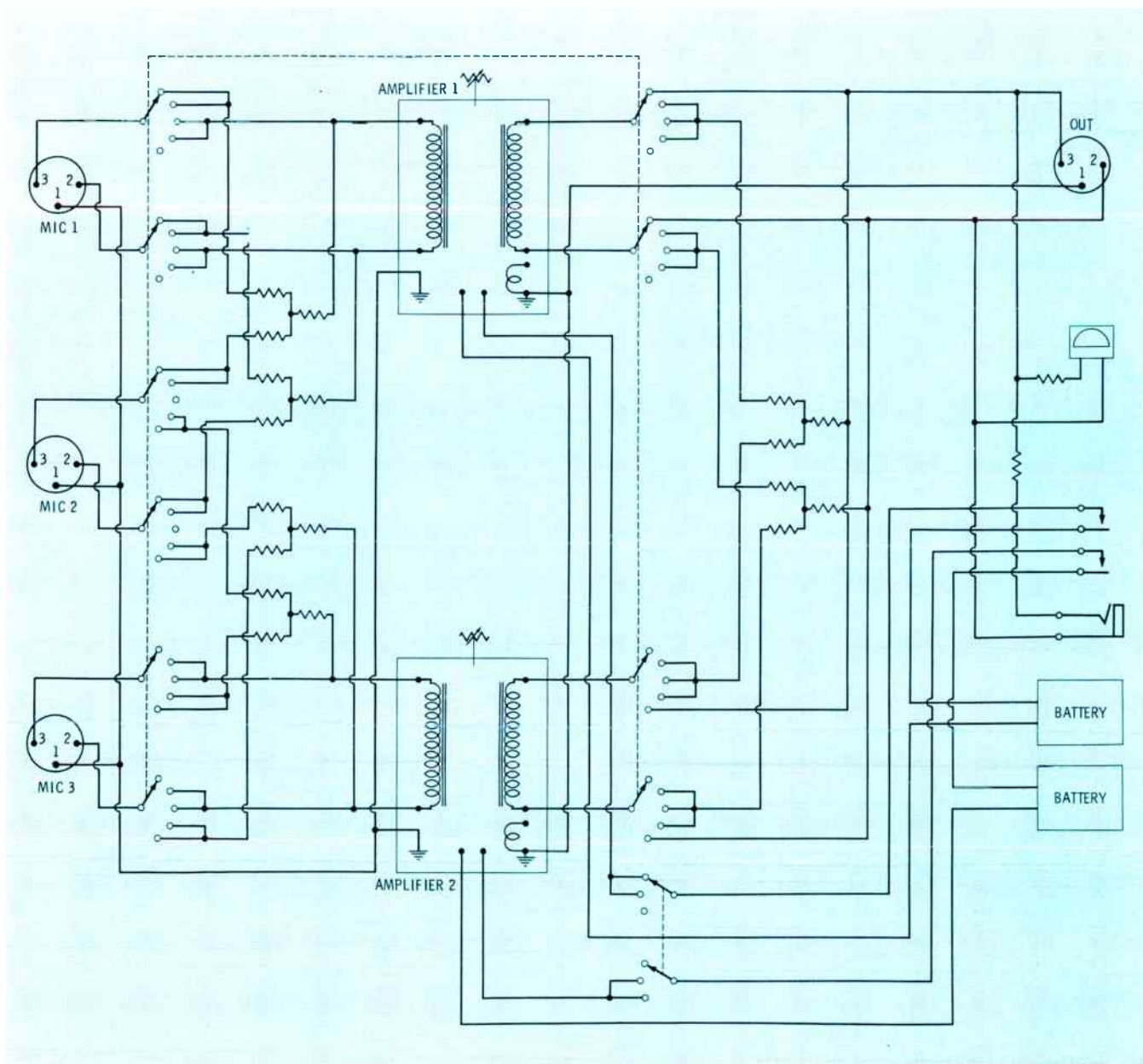
Fig. 3. Complete circuit of balanced redundant amplifier provides sophisticated operation with one ten-gang switch.
