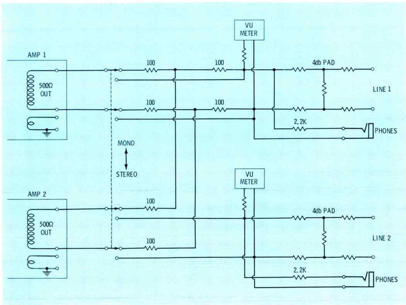
Fig. 4. Output circuit of the redundant remote amplifier modified for operation in monophonic or stereophonic mode.
