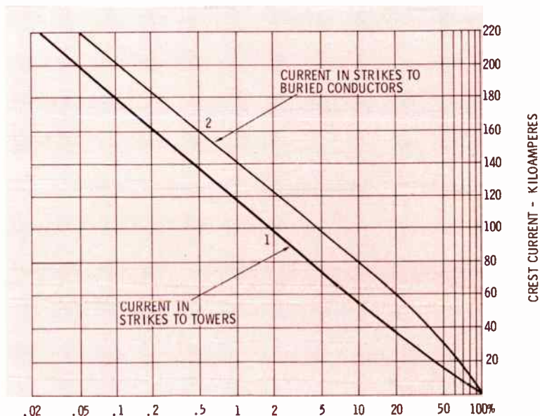
Fig. 1. Curves show percentile of lightning strokes in which the stroke current exceeds the ordinate. The curves represent the maximum current which occurs during the stroke.
