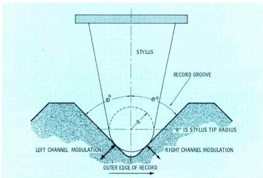
Fig. 4. Geometry of stereo record groove shows how stereo effect is achieved.
