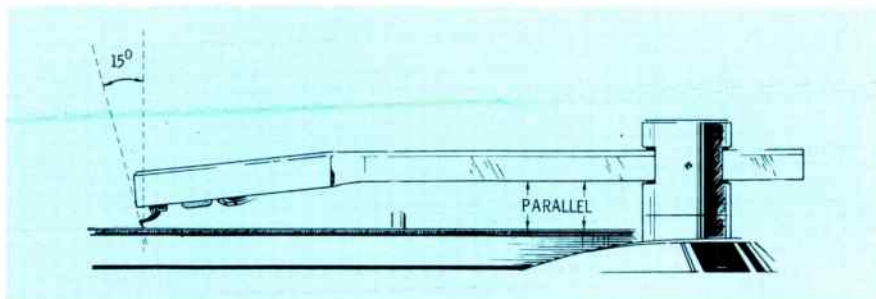
Fig. 3. Vertical tracking angle requires cartridge shell to parallel disc.
