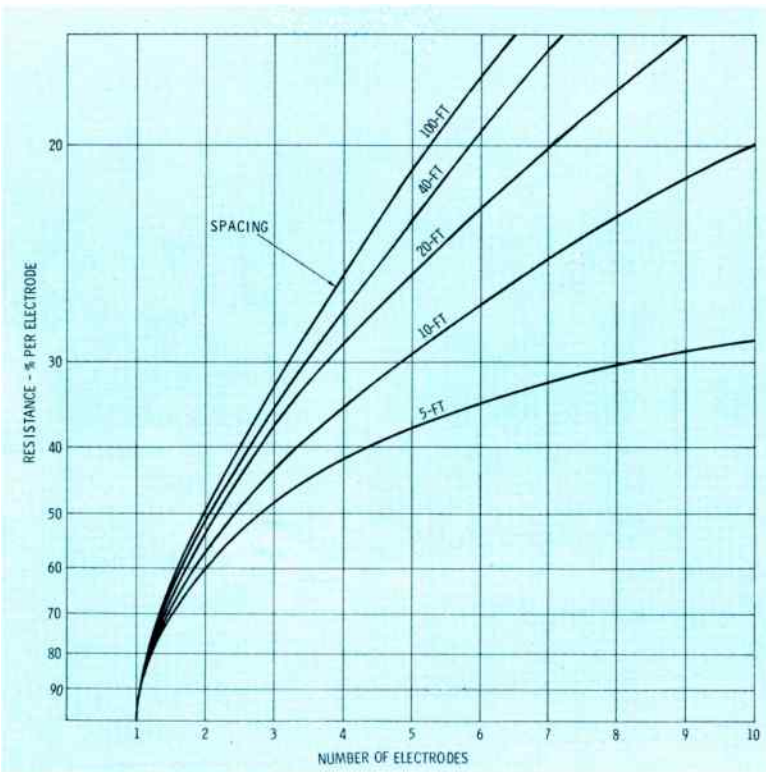
Fig. 3. The number of electrodes and the spacing between them both contribute toward the efficiency of a ground system which employs driven copper rods or tubes as its elements.
