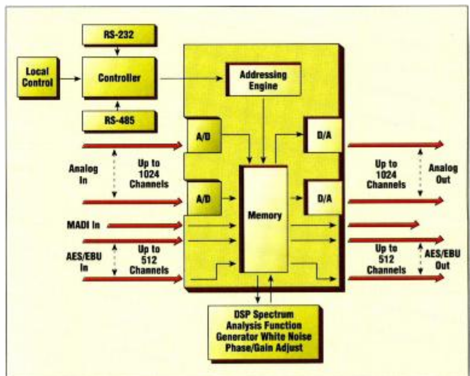
Figure 1. Simplified OZ Block Diagram
