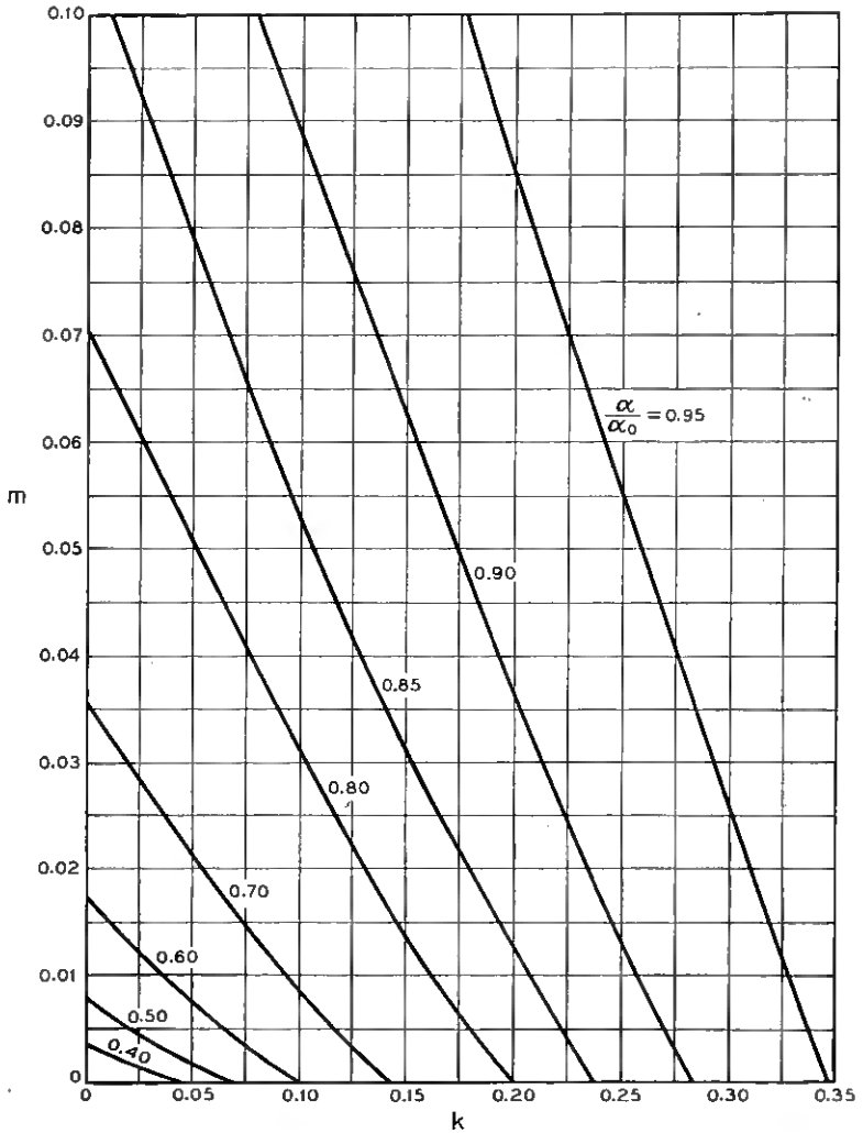
Fig. 6 — The relation between dielectric loss parameter m and magnetic loss parameter k for which the maximum possible reduction of attenuation is the same, plotted for several different values of attenuation reduction.
