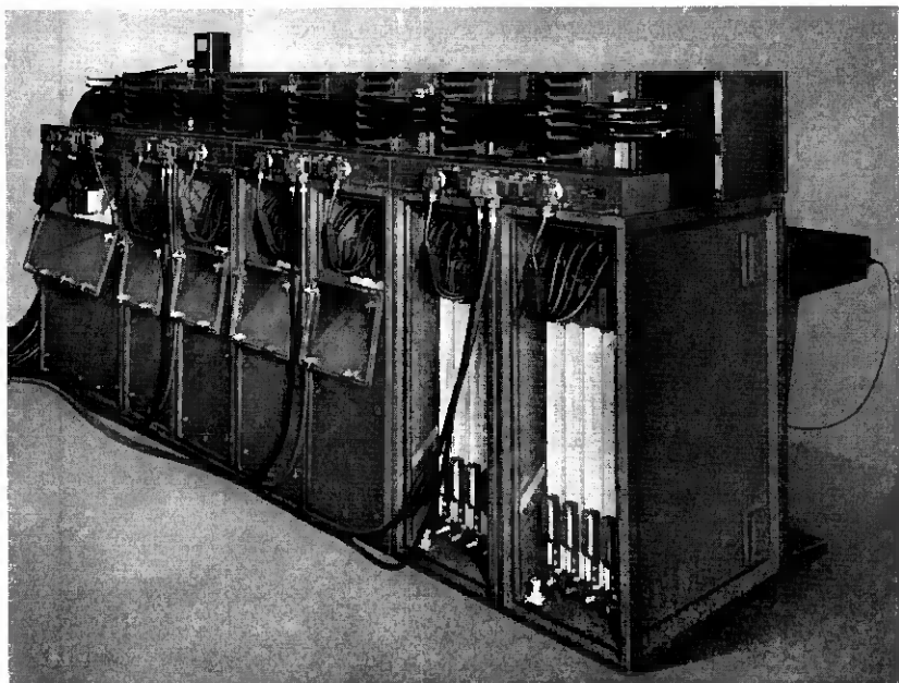
Fig. 4 — Rear view of switchboard position line-up. The right-hand position has both half-section rear covers removed to display the manner in which cord packs are mounted in position cases. The line and trunk multiple mounted on the top front of the position cases shows the orderly manner in which multiple cables are racked.
