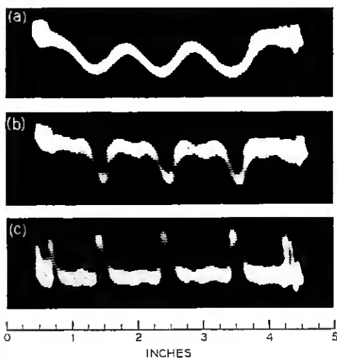
Fig. 11 — Photograph of pulses on the television monitor.
