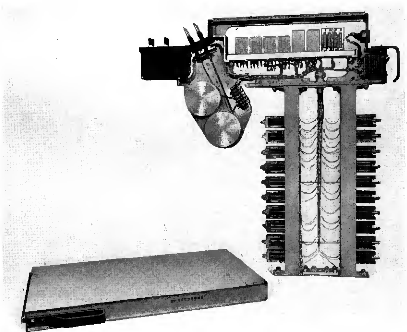
Fig. 5 — Switchboard cord pack containing two cord circuits with the dust cover removed.
