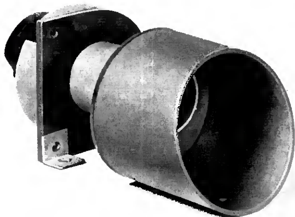
Fig. 4 — Sound radiator of the tone ringer.
