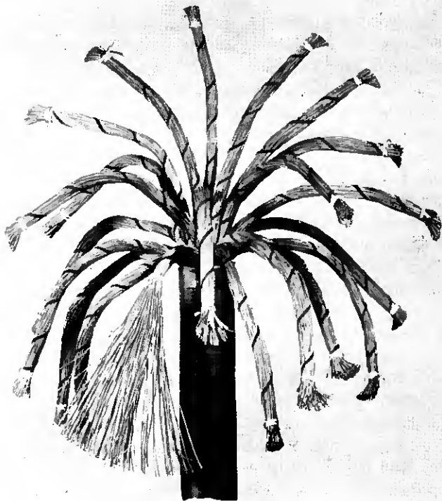
Fig. 8 — Multiple-unit telephone cable, consisting of 21 groups, each comprising 101 pairs of 26-gauge wires.
