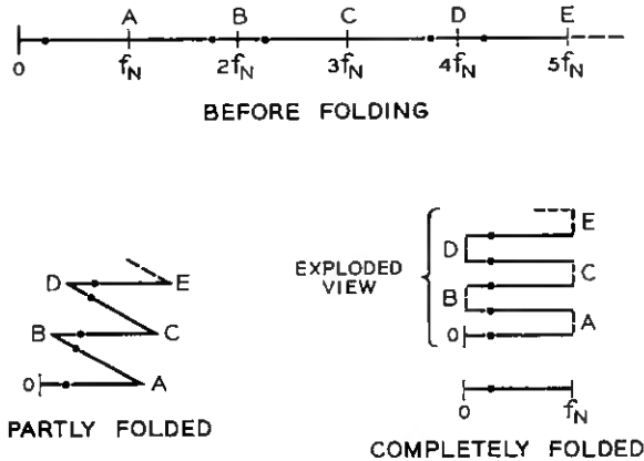
Fig. 18 — Spectrum folding.
