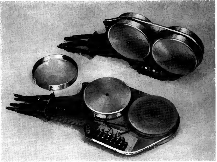
Fig. 10 — Cord reel assembly showing the switchboard cords in the retracted position. This assembly provides access to two cord circuits.
