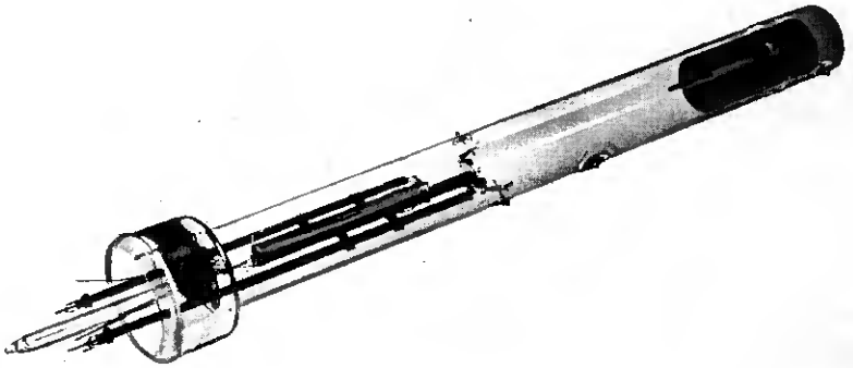
Fig. 1 — Photograph of broadband oscilloscope tube — Model III.
