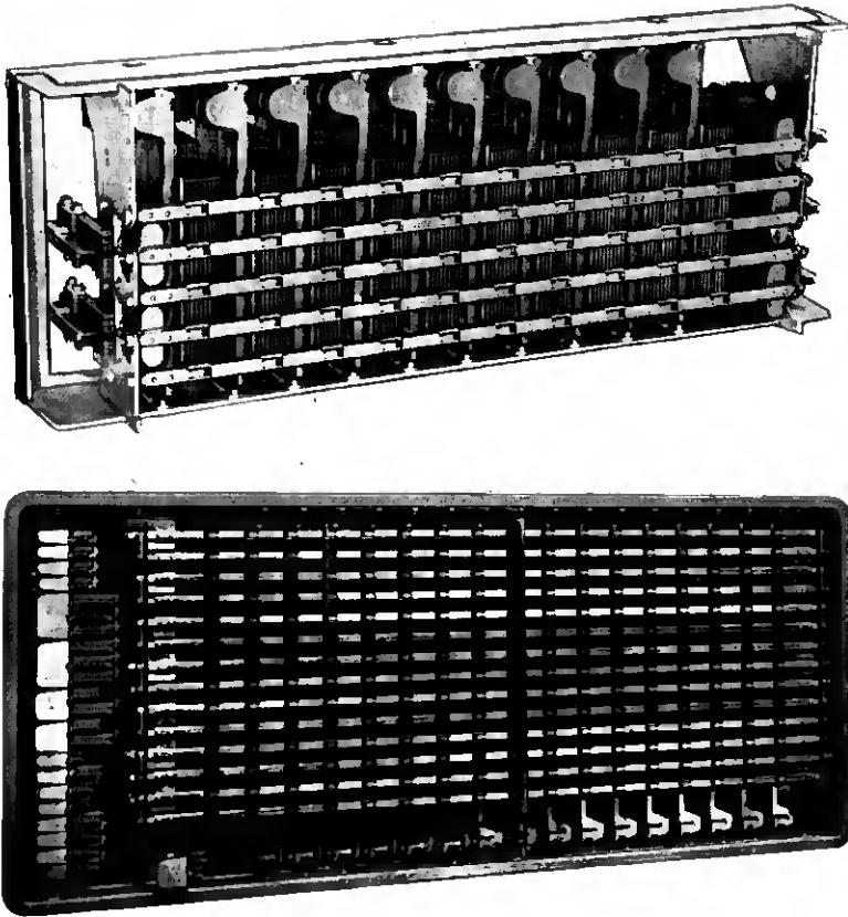
Fig. 17 — Top : Crossbar switch, present date design by the Swedish Telecommunications Administration. (By courtesy of Swedish Board of Telecommunications.) Bottom : "Pentaconta" crossbar (France). (By courtesy of International Telephone and Telegraph Co.)
