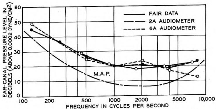
Fig. 6—Ear canal pressure level for certain reference conditions. The measurements for the M. A. P. curve were made nearer the ear drum than those for the other curves. See text.
