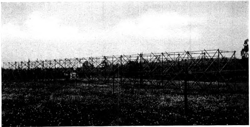
Fig. 18—Bruce receiving antenna at Netcong, New Jersey, used for transoceanic communication. This type of antenna has been superseded by the rhombic type at Netcong.
