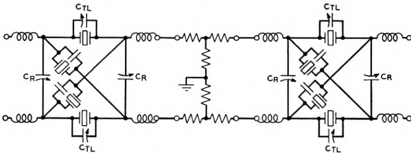
Fig. 13—Schematic of crystal channel filter.
