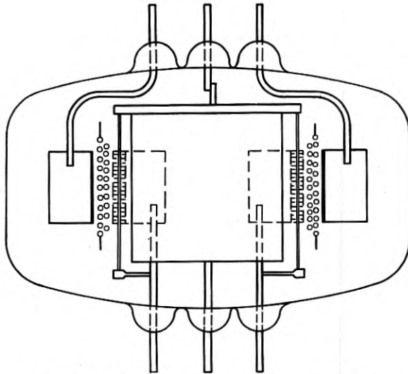
Fig. 4—Section view of the double pentode tube.
