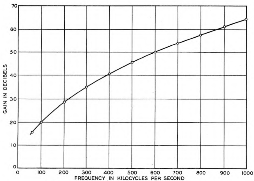
Fig. 7—Gain-frequency characteristic of coaxial repeater.
