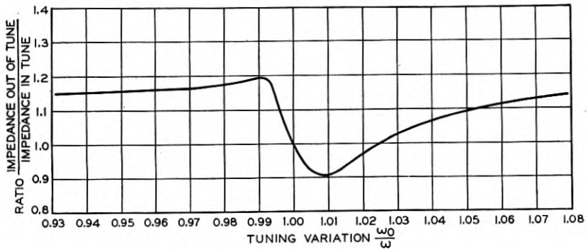
Fig. 15—Reaction curve.
