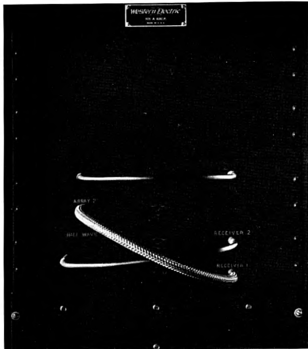
Fig. 22—An experimental radio-frequency jack board terminal for small concentric-tube lines. Path cords are constructed in the manner depicted in Fig. 21.
