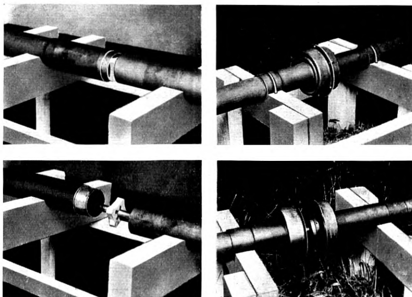
Fig. 19—Experimental expansion and lock joints for large sizes of concentric tube line.
