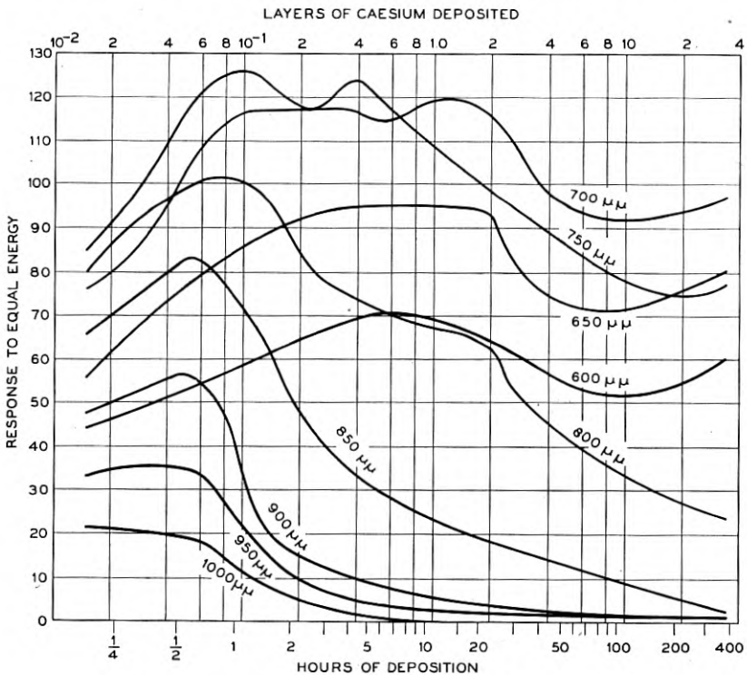
Fig. 16—Spectral response changes in cell F , position 2.
