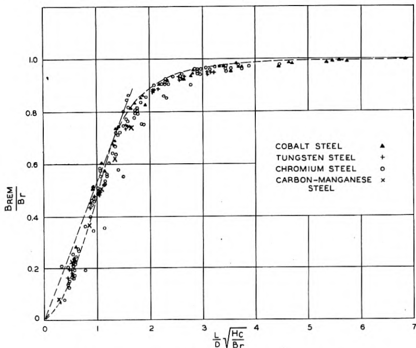
Fig 6.—The data of Fig. 4 with B_{rem}/B_r plotted against L\sqrt{H_c}/D\sqrt{B_r} .
