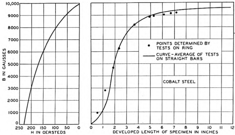
Fig. 8—Comparison of B_{rem} vs. length curves for straight bar and 2-in. I.D. ring of \frac{1}{4} -in. x \frac{1}{4} -in. cobalt steel in which B_r = 9,980 gauss and H_c = 230 oersteds.
