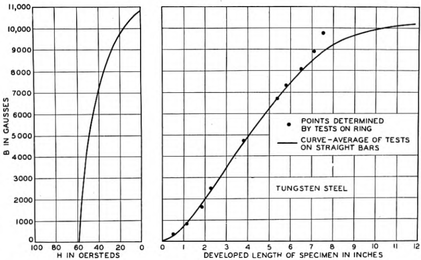
Fig. 9—Comparison of B_{rem} vs. length curves for straight bar and 2-in. I.D. ring of \frac{1}{4} -in. x \frac{1}{4} -in. tungsten steel in which B_r = 10,830 gauss and H_c = 59 oersteds.
