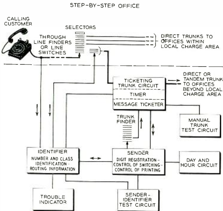
Fig. 1 — Block diagram of the automatic ticketing system.
