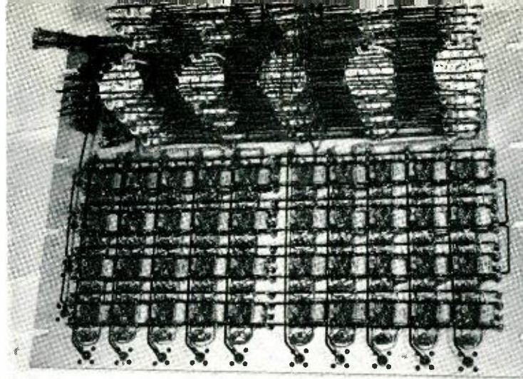
Fig. 2 — The transistor gating matrix. The array of switches in the background is the Target-by-p-Computer switch of the gunnery system simulator.
