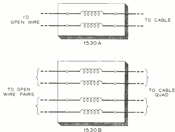
Fig. 6 — Schematic diagrams of the new inductors. Protectors on the open-wire side are not shown.
