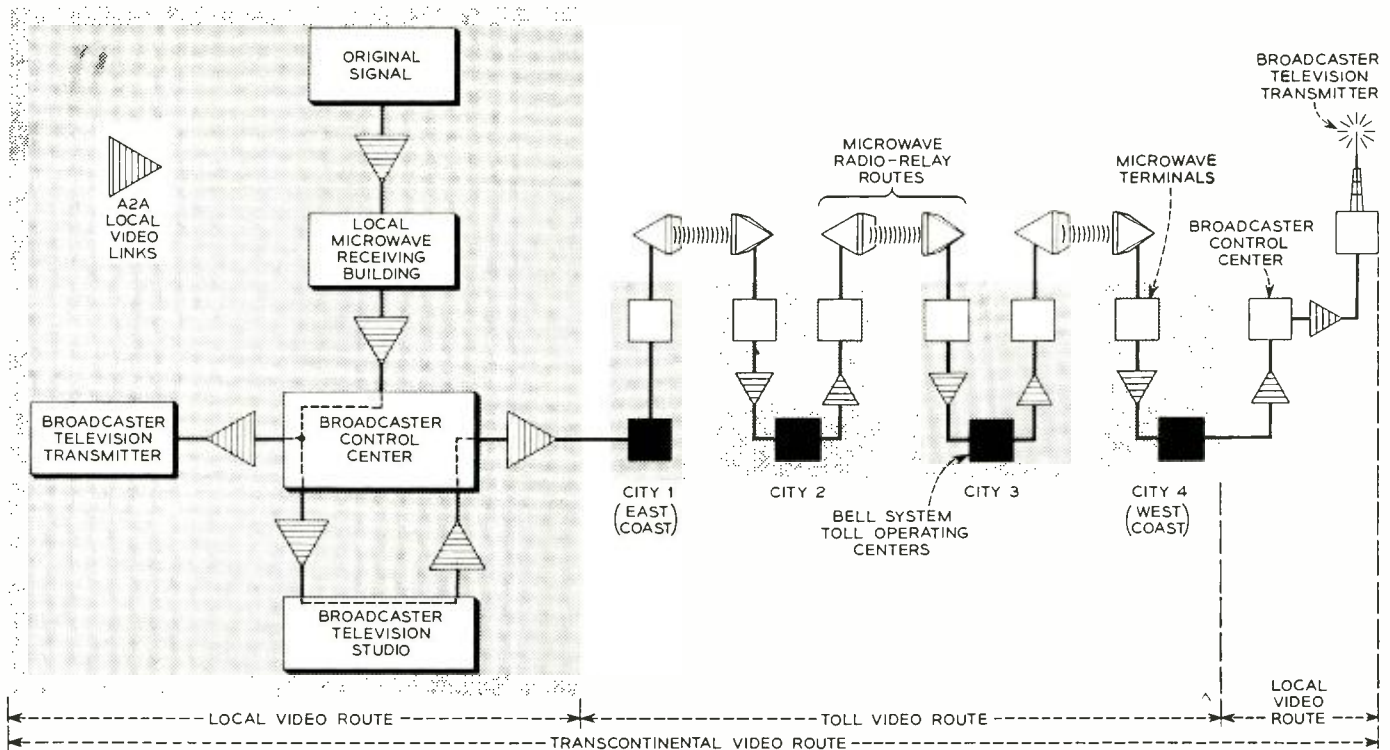
Fig. 1—Left, typical intra-city television network, showing how several A2A links might be used; right, typical coast-to-coast television hookup, showing role of numerous A2A links in over-all connection.
