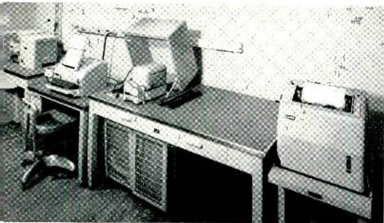
Fig. 1 — Remote operating station and storage input tables for the Network Problem Computer (Model VI). Originally installed at the Murray Hill Laboratory in 1949.
