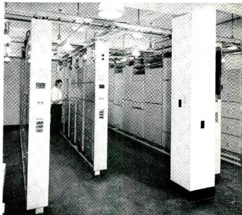
Fig. 3—Relay equipment room of the Model V Computer installed at Ballistics Research Laboratories, Aberdeen, Md.
