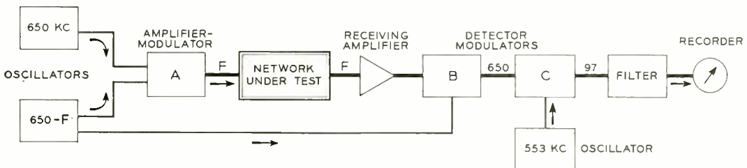
Fig. 3—Block diagram of automatic transmission measuring circuit.
