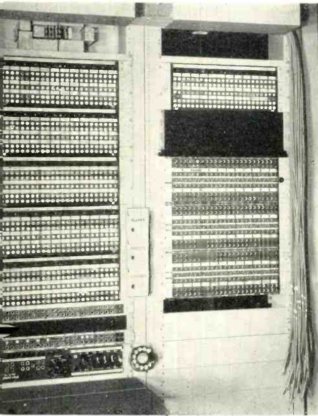
Installation of 482A and 410A jacks at Newark.
