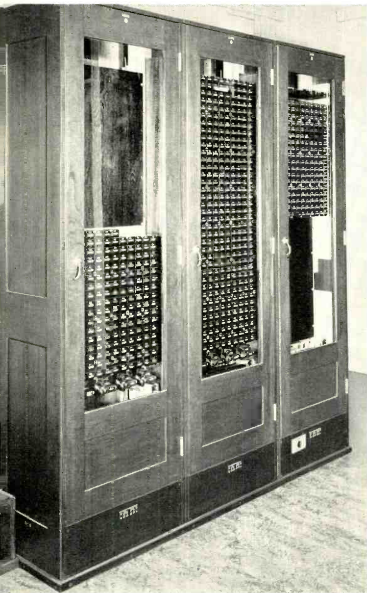
Fig. 2—Left, a traffic register cabinet of the earlier type. Right, part of a traffic register distributing frame.
