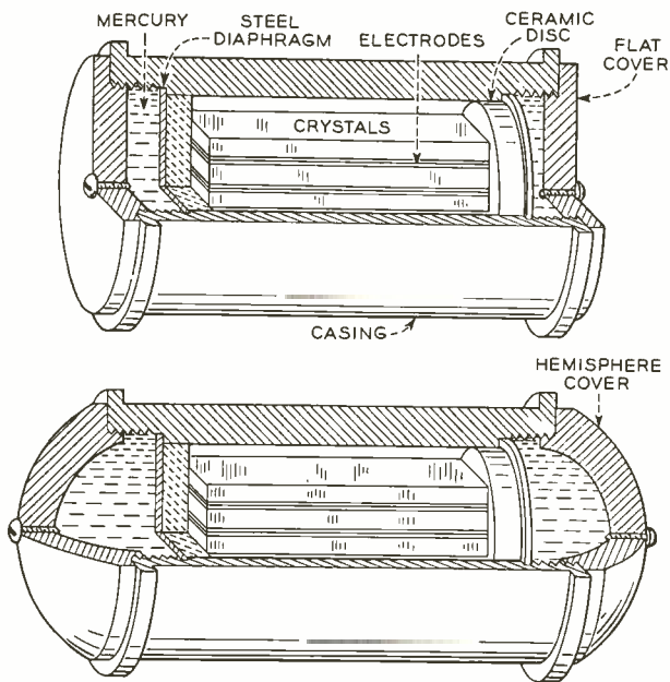
Fig. 2—Simplified cross-section of accelerometer unit for submarine cable repeater, above, and a similar accelerometer but designed for measuring accelerations in any direction, below.
