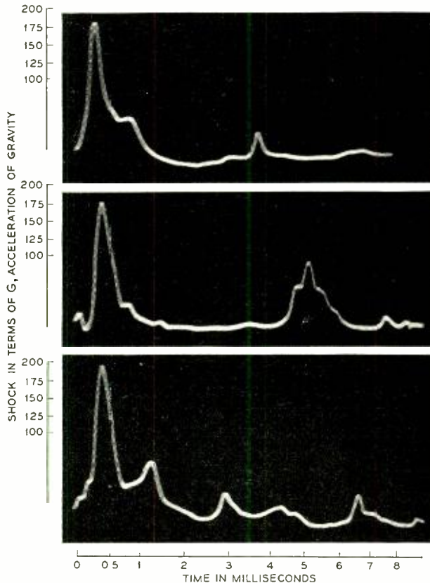
Fig. 3—Typical handling shocks experienced in tests at Bell Telephone Laboratories. Top—a 180g shock merged with a smaller secondary shock probably due to the cable's not striking uniformly along its length. (A small secondary shock is also present.) Middle—a 170g shock in which the cable appears to have struck evenly, producing a rather smooth shock followed about four milliseconds later by a second and smaller shock. Bottom—a 200g shock of approximately \frac{1}{4} millisecond duration followed by considerable secondary vibration. In all three oscillograms, the cable was traveling from 80 to 100 inches per second, and thus 4 or 5 milliseconds corresponds to a travel of less than half an inch. All secondary shocks are thus attributable to the first impact and not to bouncing of the cable.
