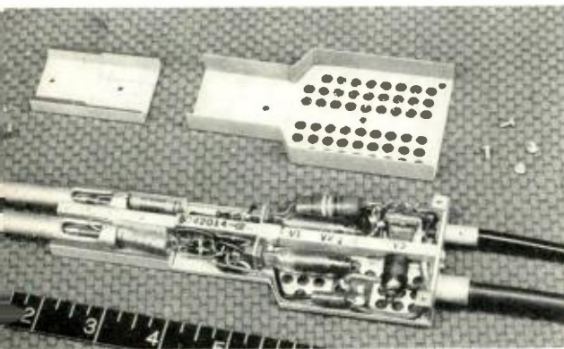
Fig. 1—The high impedance video monitoring probe with its cover removed.
