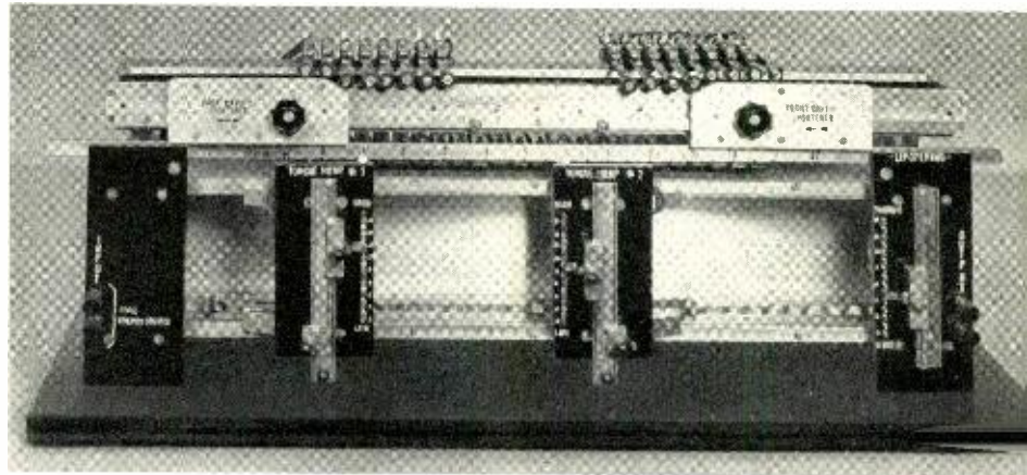
Fig. 5—Close-up of the vocal tract of the analog vocal system.
