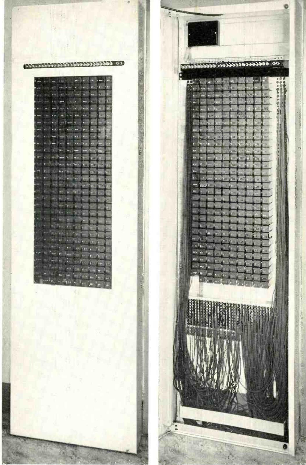
Fig. 1— Left, one of the new traffic register cabinets with doors closed. Right, opening the door of a traffic register cabinet gives access to the cords by which the various registers are connected to the required circuits.
