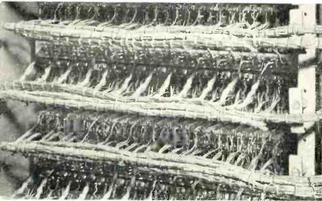
Left—Sewn cable forms at the rear of the four-wire voice frequency bay equipped with 410A jacks. Right—Use of new fanning strips with the 482A jacks provide greater accessibility as well as neater appearance at reduced cost.
