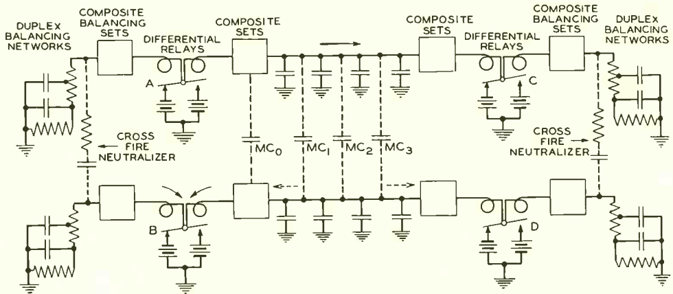
Fig. 1—Telegraph circuits formed from the two sides of the talking channel, showing the various capacitances and balancing networks
