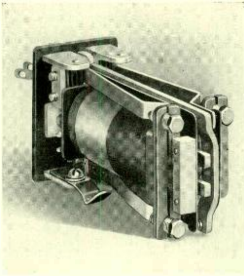
Fig. 6—The weight attached to the contact arm of the pendulum J relay is clearly evident in the photograph
