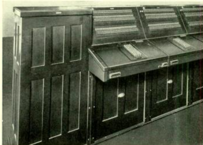
Fig. 1—Each position of the older type of "B" board is equipped with keys and lamps for sixty trunks, and a key set of forty keys for "writing up" the number called
