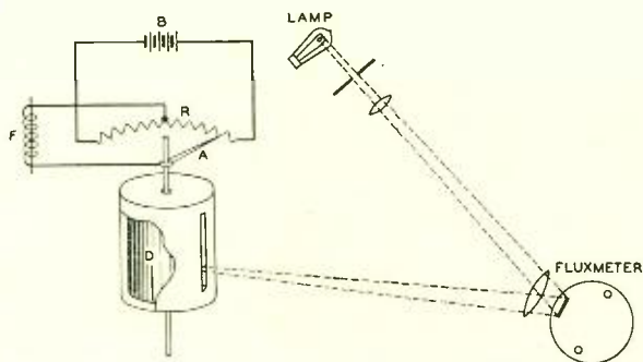
Fig. 2—The graph is made on a sheet of sensitized paper fastened to a drum, the rotation of which varies the exciting field of the specimen
