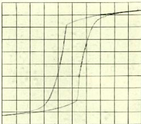
Fig. 3—Hysteresis loop of permalloy containing 78.1% nickel made on the new apparatus
