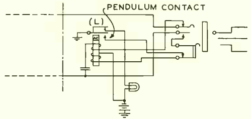
Fig. 5—Use of the pendulum J relay brings in a time element which avoids false locking of the L relay
