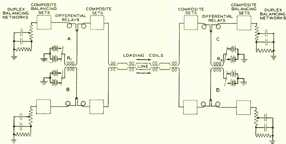
Fig. 3—Coupling between conductors through the loading coils is the cause of the greater part of the receiving-end crossfire
