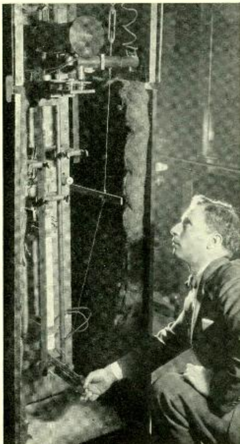
P. P. Cioffi operating device, sensitive to four parts in a billion, for determining changes in length of magnetic materials with magnetization
