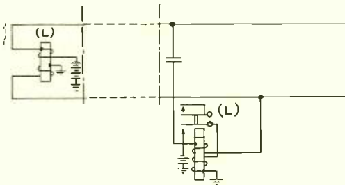
Fig. 3—By changing the polarity of the locking winding with respect to the operating winding the effects of the various surges may be reduced. Inner ends of windings are indicated by a semi-circular dot
