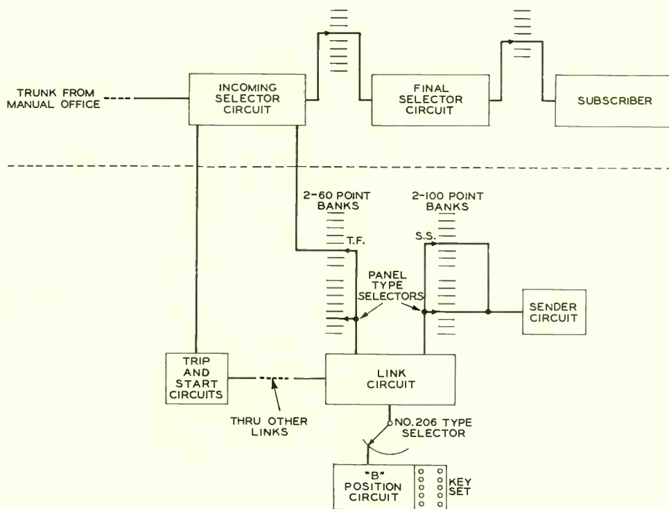
Fig. 3—Schematic diagram for call-distributing "B" board
