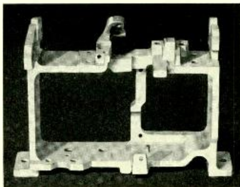
Fig. 5—Frame of step-by-step switch with sherardized finish
