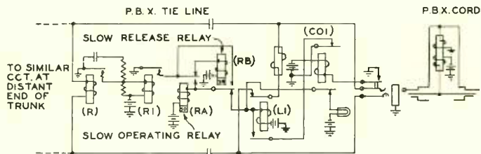
Fig. 7—A circuit that prevents transient surges from lighting the operator's line lamp uses a train of four relays, one of which is slow operating and one, slow release
