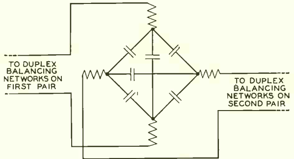
Fig. 2—The compensating network to neutralize sending-end crossfire makes connection to all four conductors of a quad
