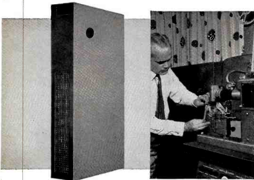
G-E Scanner Pickup —serves the same function as the film camera now used with B & W projectors. Dichroic mirrors break the light from the projectors into primary colors—photo-electric pickup cells convert it to electric signals.
