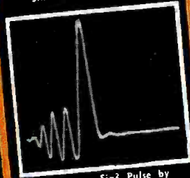
Effect on Sin 2 Pulse by NTSC phase equalizer. Check for transient response of a unit or system—Model 1073-A.
