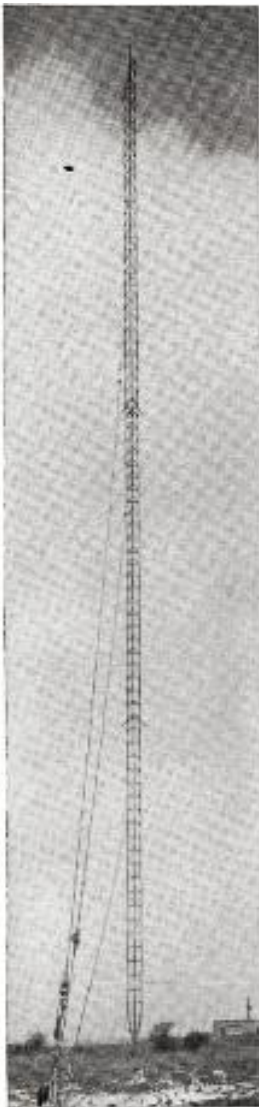
WFMJ-TV Truscon Triangular Guyed Tower 1000-Feet Tall
