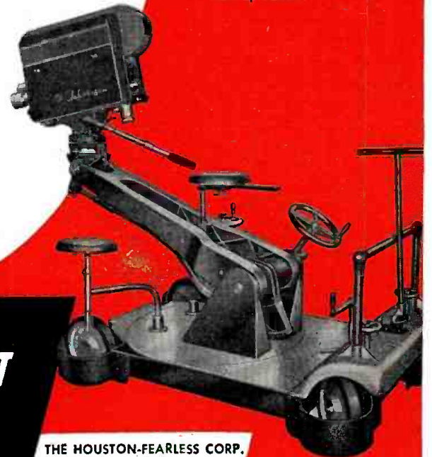
H-F Panoram Dolly provides countless camera effects . . . raising, lowering, panning, tilting, and dollying. Smooth and steady.
