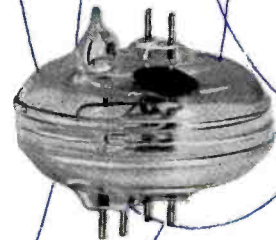
1940. The beating oscillator, used in the great majority of radar systems. This tube generated a wave in the receiver with which the received microwave was reduced in frequency for amplification.
