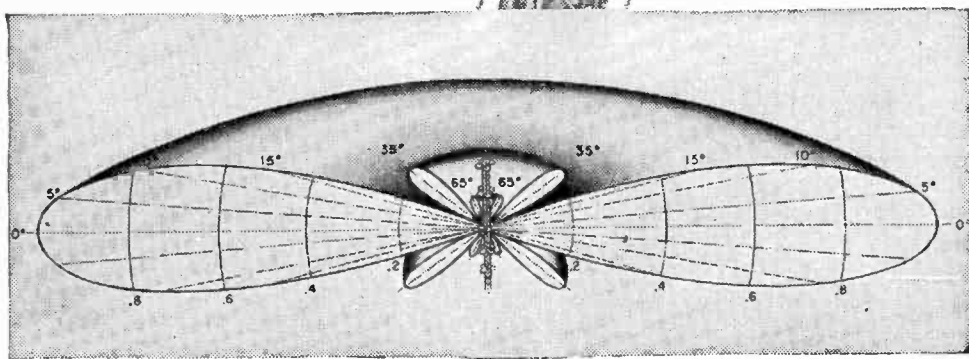
Radiation Pattern for 5 unit array.
