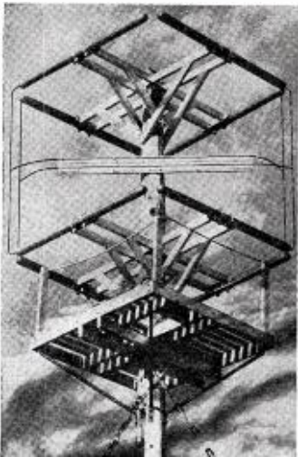
NEW cubical type antenna has been developed by General Electric engineers for use in the company's new 10,000 watt television transmitter in the Helderberg Hills, 12 miles from Albany. Built of eight hollow copper bars, each four inches in diameter and about seven feet, or one-half wave, long, arranged to form a cube, the antenna is designed to radiate a horizontal polarized wave, carrying both picture and voice on the 4½-meter band, with good signal strength for a distance of 40 miles.
