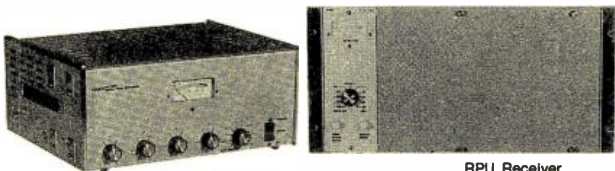
RPU Transmitter
