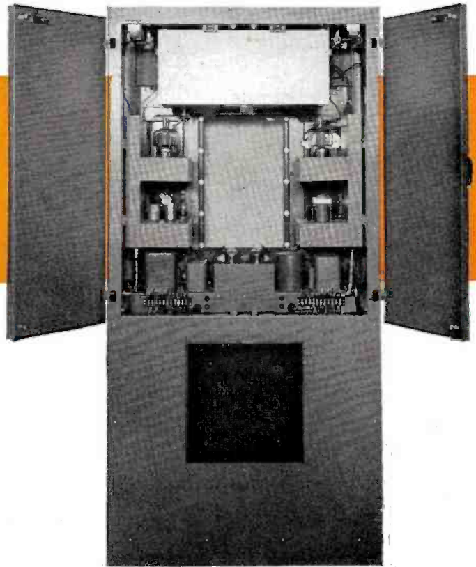
Rear, open view of the new Collins 20V 1000/500 watt AM broadcast transmitter.
