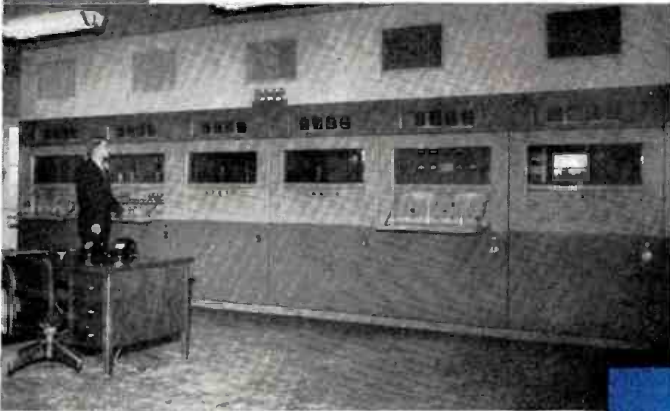
"At WDGY in Minneapolis, Minn., the Transmitter Engineer trims the RF Drive Stage of the Westinghouse 50 KW AM Radio Transmitter."
