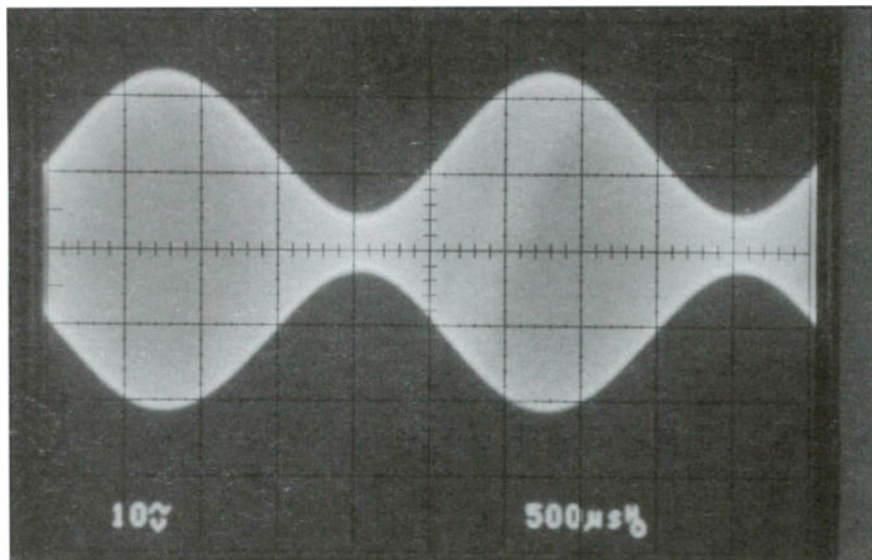
Oscilloscope image of the 455 MHz IF signal at the secondary of the last IF transformer
