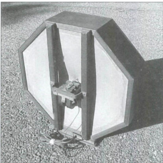
The rear of the Air-Chrome speaker showing the rear unpainted cone.
