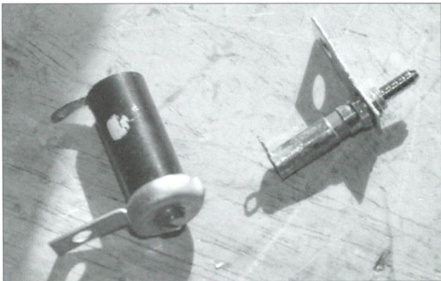
I bet some of you recognize the damn piston capacitor above used by Zenith and many more. If bottomed when adjusting the piston comes off and it has to be replaced. The better piston variable capacitor is to the right. I had to replace one in the LO 4.5-13.4MHz. Band.
