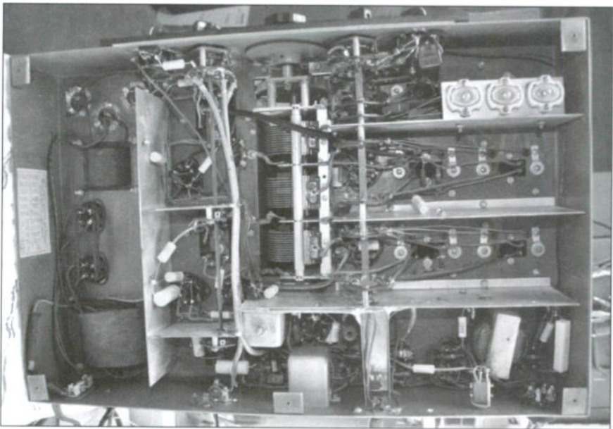
Bottom view of the McMurdo Silver chassis
