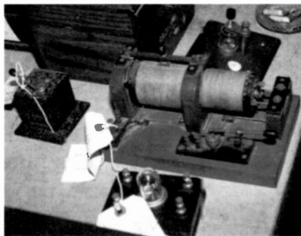
The Howe crystal set (left), sold for $35; the homebrew, loose-coupled crystal set (right), for $155; and the Philmore crystal set, (front), for $25.
