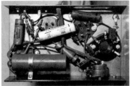
A view looking underneath the chassis of the 3-tube regenerative radio.
