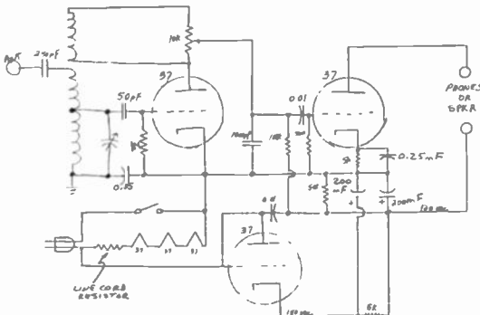
Schematic diagram for the 3-tube regenerative radio.
