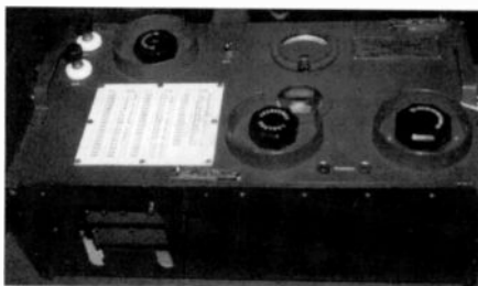
This Military Type BC0227A, manufactured by Cardwell, SN1, with Type 199 tubes, in factory new condition, sold for $1,600.
