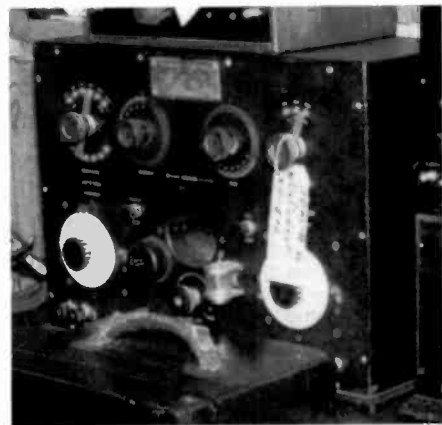
This early DeForest SP-500 receiver, with socket for exposed tube, was won with a bid of $1,200.
