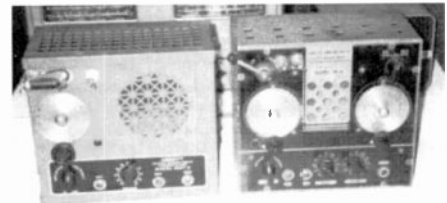
A pair of Abbott Instrument 2 1/2 meter transceivers offered in the communications auction: left, an MRT-3, and right, a TR-4.
