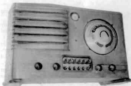
EMERSON MODEL BU-229 – One of many Emerson models in the wooden Ingraham cabinet series, this 1938 set is missing the conical dial center and the eye-tube escutcheon. It is a 7-tube receiver with broadcast and shortwave bands. ( Ralph Jackson – Northboro, MA )
