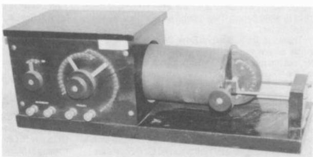
Figure 3. This loose coupler was probably made by the Wireless Specialty Apparatus Company (WSA), ca. 1918. Note that the switch for the secondary coil is rotated 90° from that of the loose coupler shown in Figure 2.
