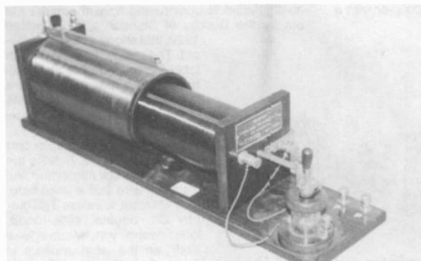
Figure 8. This excellent reproduction of a Marconi Wireless double slider tuner uses an A.H. Grebe detector. The second slider, not visible in this figure, is located at the back of the primary coil.
