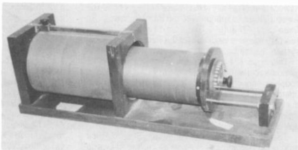
Figure 2. An example of an Arlington-type loose coupler. This unit, made by the Signal Manufacturing Company, dates to about 1919.
