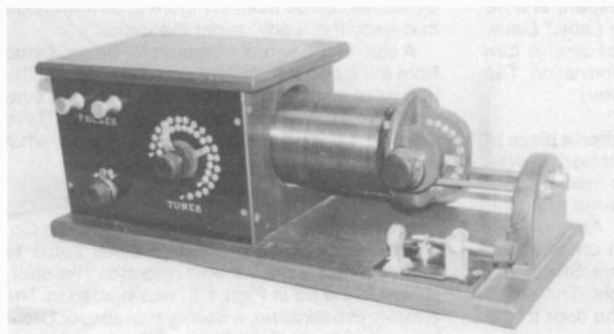
Figure 14. A replica of a Navy-type loose coupler with a SORSINC crystal detector.
