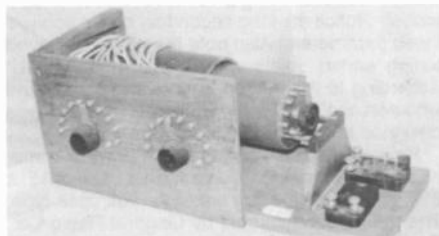
Figure 6. An example of a home-brew crystal set using a Navy-type loose coupler, probably built to a U.S. Bureau of Standards publication, with a Murdock phone condenser and crystal detector.
