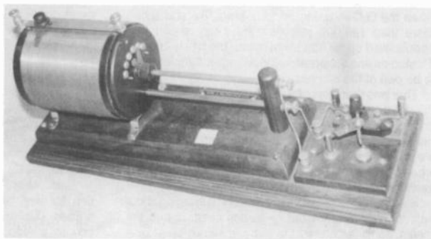
Figure 1. This nice crystal set consists of a Murdock loose coupler and a crystal detector by Montgomery Ward. The Murdock nameplate is partially visible at the rear of the wooden base.
