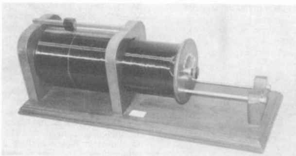
Figure 12. An example of the Arlington-type loose coupler, this is a reproduction of a loose coupler produced by the Electro Importing Co.
