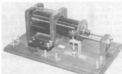
Figure 5. Another reproduction loose coupler with a convincing "old look."
