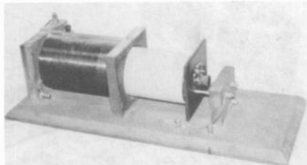
Figure 7. This basic Navy-type loose coupler is a reproduction I put together some time ago. It is an Arlington type of coupler using a rather long length of fine wire on the moving coil.
