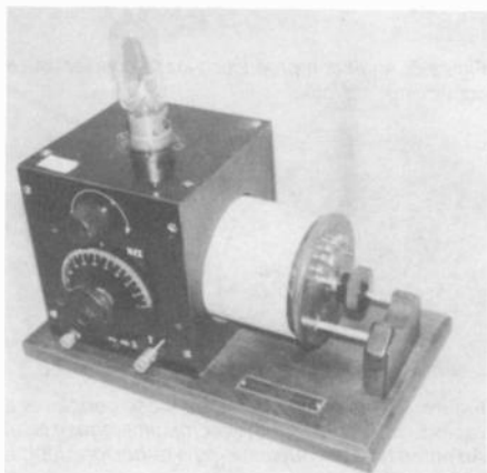
Figure 10. A very convincing reproduction of a Bruno Model BRU No. 3, a loose coupler with a ED-11 detector.
