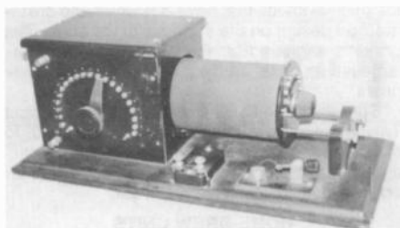
Figure 4. This reproduction loose coupler was made in 1939 and copied from a 1914 model.
