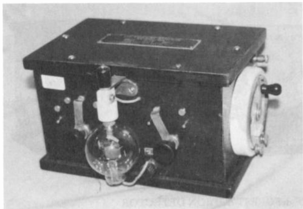
Figure 3. The De Forest RJ4 detector. (A repro tag has been added to the top. It was necessary to substitute the part above the tube socket.)
