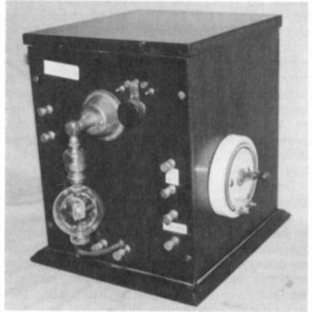
Figure 1. An unusual version of the De Forest RJ5 detector which underwent significant restoration. (The white paper tags on this and all other items are for owner purposes.)
