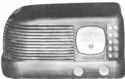
ZENITH MODEL 4B314 – This 1939 farm radio, operated by a 6-volt battery, uses a vibrator in the power supply — unusual for a table model. A 4-tube set, it uses Types 6A8, 6K7, 6Q7, and 6G6. The cabinet is brown Bakelite with white knobs. (Herbert Eltz – Juniata, NE)
