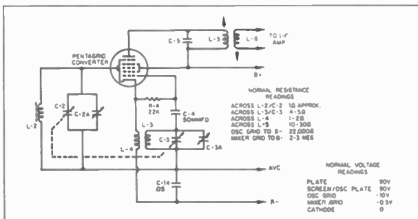
Figure 7. Schematic of ac-dc table radio converter stage.
