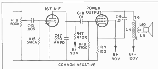
Figure 5. Schematic of standard ac-dc radio audio circuitry.
