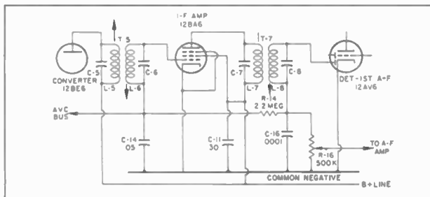
Figure 6. IF, detector and AVC stage circuits.
