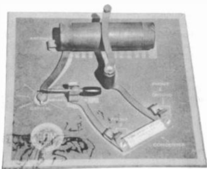
EAM TOY CO. CRYSTAL SET – This quaint little "breadboard" style crystal radio is mounted on a masonite board with yellow painted trim and component positions. The hardware is constructed of brass. ( David Petrozello – Johnson City, NY )
