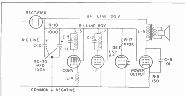
Figure 4. B+ distribution circuits for typical table model radio.
