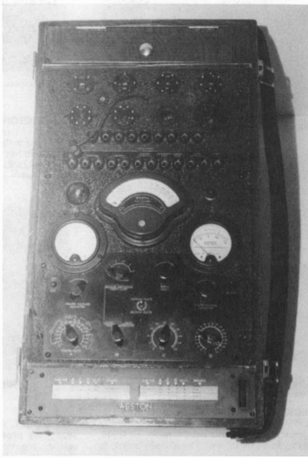
Figure 1. The "great" in size and quality Navy OQ-3 tube tester with (count 'em) 21 banana jacks!
