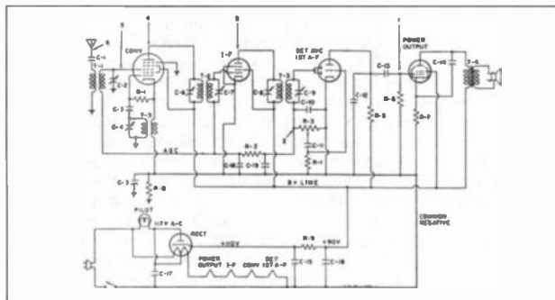
Figure 2. Schematic of typical ac-dc receiver.
