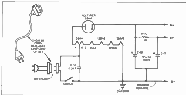
Figure 3. Power supply and filament schematic for ac-dc radio.
