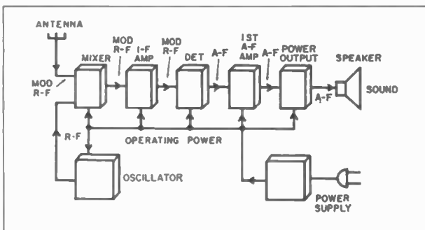
Figure 1. Block diagram of typical ac-dc receiver.
