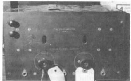
These early units from obscure manufacturers brought surprisingly high prices. The Home Manufacturing Company of Jersey City 3-tube detector and 2-step amplifier at left sold for $750; the Lawsam Electric Company RA-7 2-stage amplifier, at right, for $350. (Terrey photos)
