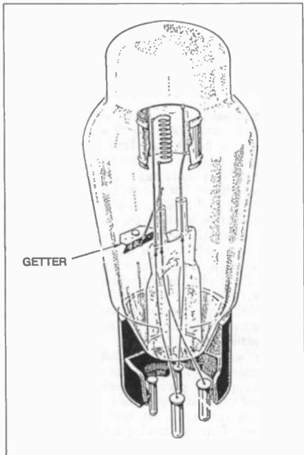
Figure 1. The getter is shown here inside the glass envelope of a standard-shaped vacuum tube. (Photo from "How to Repair Old-Time Radios," p. 16.)
