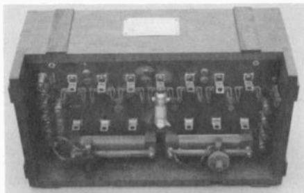
A British Marconi Type 55 amplifier using seven V24 tubes, one of which can be seen in the center. (McElroy photo)
