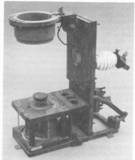
A Telefunken Type E-5 crystal receiver, ca. 1914, missing the detector and other parts. (McElroy photo)
