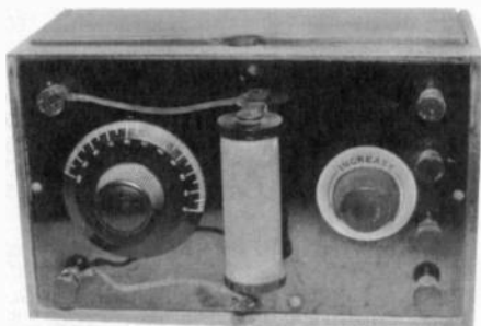
MIRACO MODEL UNKNOWN – This 1-tube radio was made by the Midwest Radio Corporation of Cincinnati, Ohio, in about 1923. An unusual feature is the front-mounted loading coil. Originally, there was a decal on the front panel with the MIRACO logo. (Greg Farmer – Fridley, MN)
