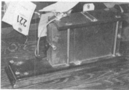
A Murdock variable capacitor using sliding rectangular plates. (Terrey photo)
