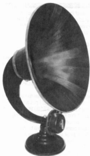
RADIO CABINET CO. ORCHESTRION – This Burns horn speaker has a very unusual wooden bell. The bell is obviously made by Radio Cabinet Co. (Orchestrion). I have located two others like this. Are there more? (Ed Bell – Raleigh, NC)
