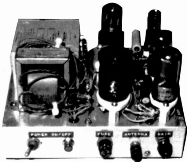
Figure 2. A modified AM broadcaster — the final product!
