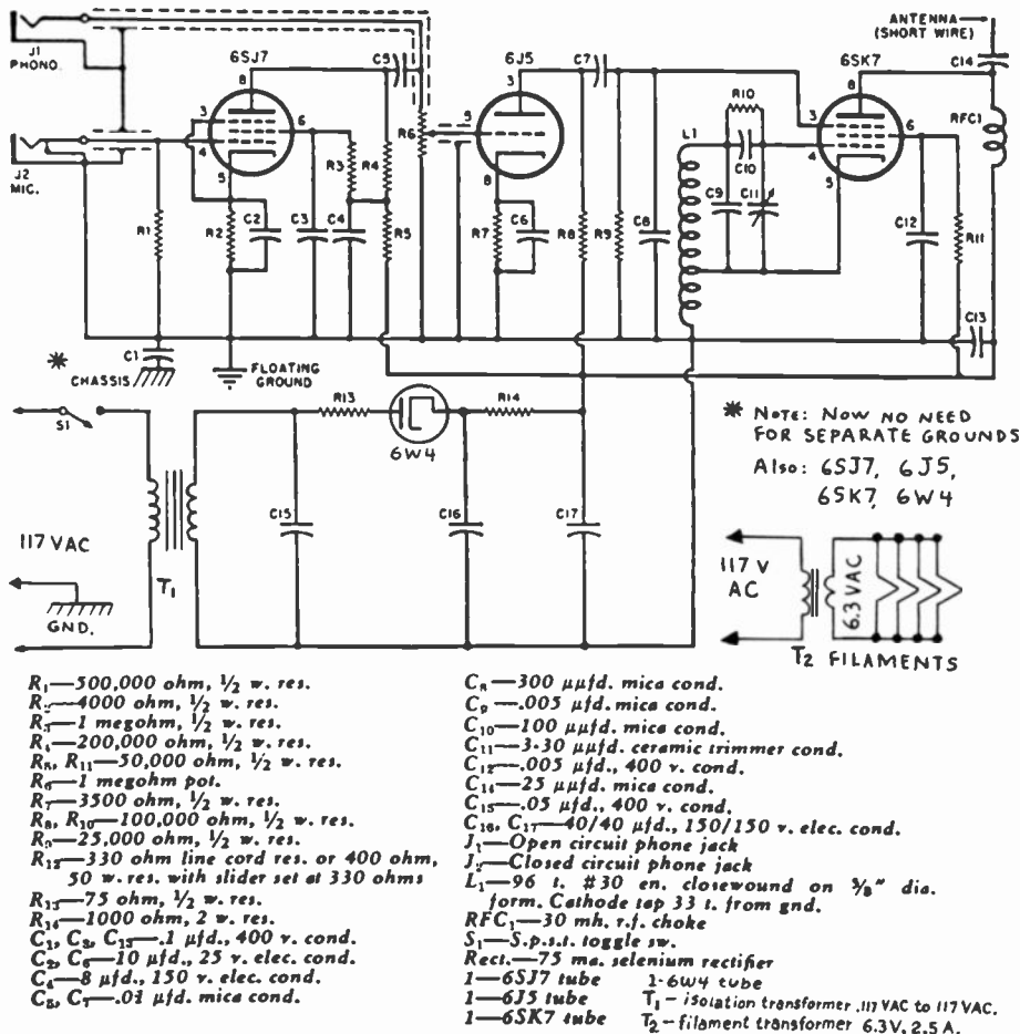
Figure 1. Modified schematic for AM broadcaster, from "Radio News," October 1947.
