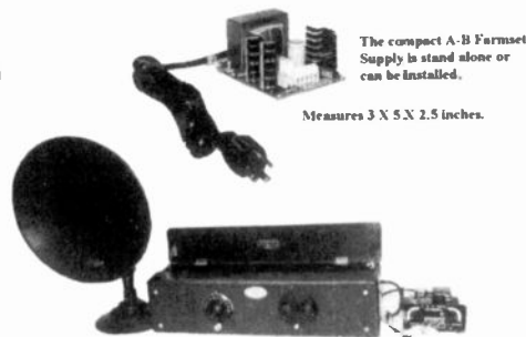
An Atwater Kent Model 33 being powered by the A-B-C Benchtop Supply (Right) Measures 5.5 X 7 X 3.5 inches.
