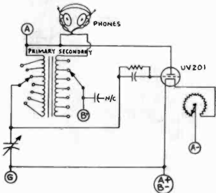
Figure 4. Schematic of the Type 2A receiving set.
