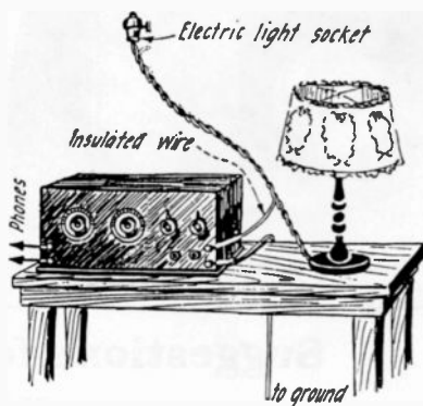
Figure 1. Illustration of House Wiring Antenna from "Radio News," April 1924, p. 1437.
