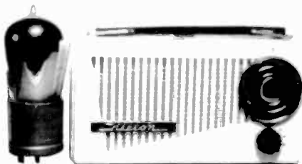
HILTON MODEL G. W. 3672 – Measuring 2" by 3 1/2" by 6", not much larger than a Radiotron UV 201 tube, this tube-type superhet portable contains 4 miniature type tubes — 1T4, 1R5, 3S4, and 1U5 — plus a dynamic speaker. For power, it has a 1 1/2 volt C cell and a 45-volt Eveready Type 415 B battery. The small knob switches to a low, high, or earphone position. (Richard Buchan – Sun City, CA)
