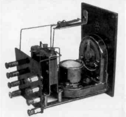
Figure 7. The chassis of the Type 3B amplifier showing the molded socket and rheostat unit.
