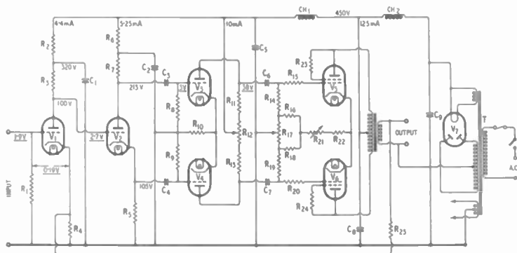
Circuit diagram of complete amplifier. Voltages underlined are peak signal voltages at 15 watts output.
