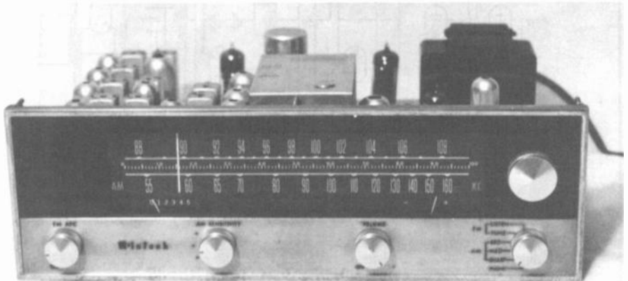
Figure 3. McIntosh Model MR55A, an early monaural tuner.
