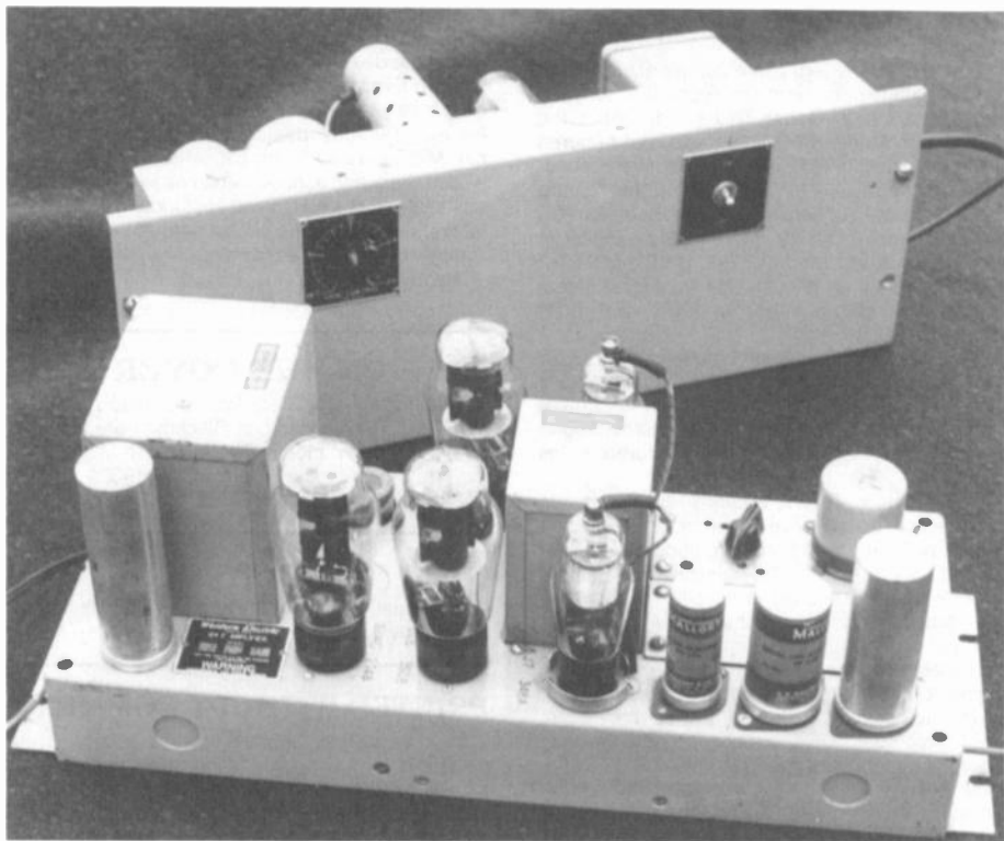
Figure 1. Western Electric Model 124E amplifier.
