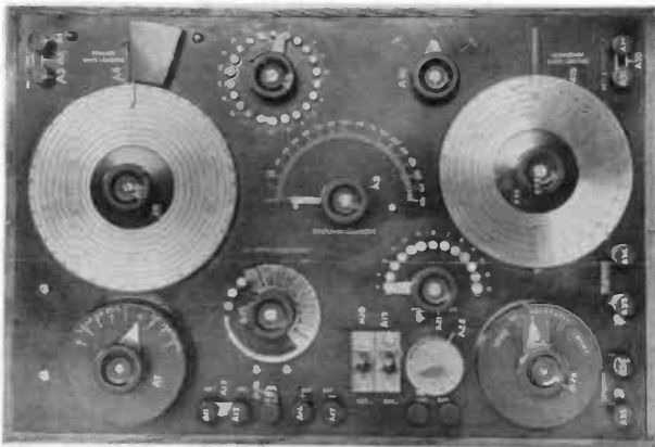
Figure 7. Cohen Type A receiver. (Reproduced from Bullard, Figure 528, opposite p. 708)
