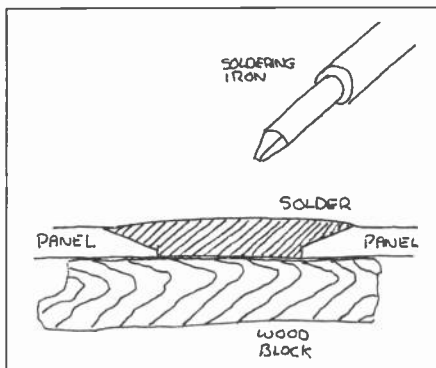
Figure 2. Fill hole completely with solder.
