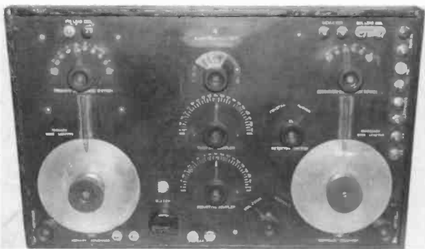
Figure 19. The SE-998 shortwave receiver. (Photo from the W. Jensby collection)
