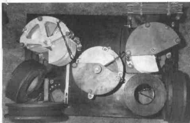
Figure 11. Internal view of the Type B A receiver.
