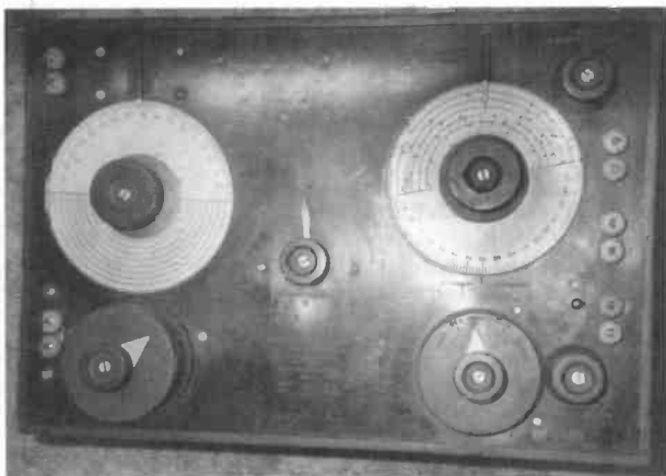
Figure 10. Front view of the Model B A receiver.
