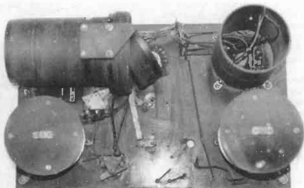
Figure 14. SE-143 receiver, internal view.
