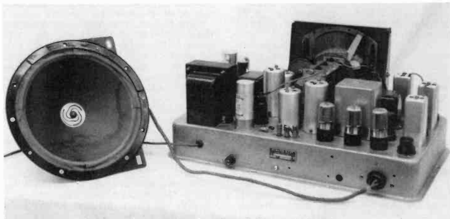
Figure 2. Rear view of AK 810 chassis, with Type N speaker. This speaker was patented by A. D. Silva.
