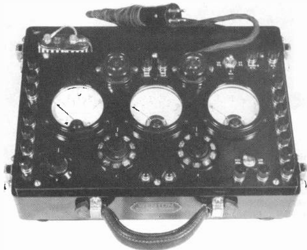
Figure 1. The Weston 547 Radio Set Analyzer.
