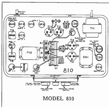
Figure 4. Tube layout chart from "Rider's Perpetual Troubleshooter's Manual, Vol. VI", page 47, showing the Atwater Kent Model 810.
