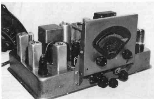
Figure 1. Front view of AK 810 chassis.
