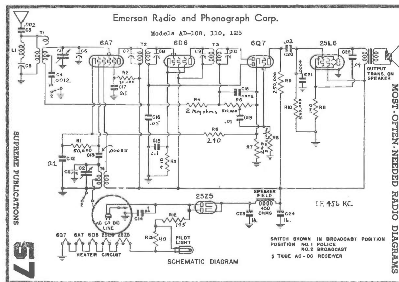
Figure 3. Wiring diagram of a typical 1930's AC/DC set.
