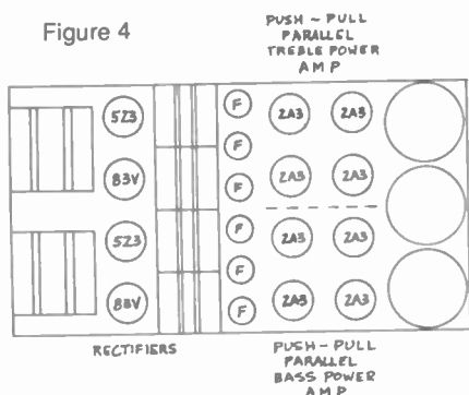
POWER AMP CHASSIS
