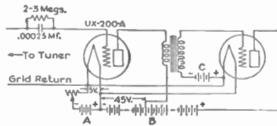
Detector, Transformer Coupled
