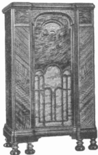
ALL WAVE—Model 318K —8-tube superheterodyne with 9 tuned circuits—complete world-wide range from 540 kilocycles to 22.5 megacycles—in 4 separate tuning bands—2-speed tuning, approximately 6 to 1 and 60 to 1 ratios—shadow tuning—six watts output—11-inch electro-dynamic speaker. Beautiful lowboy cabinet of choice veneers and matched woods with excellent acoustical properties. $89.90 f.a.b. factory.
