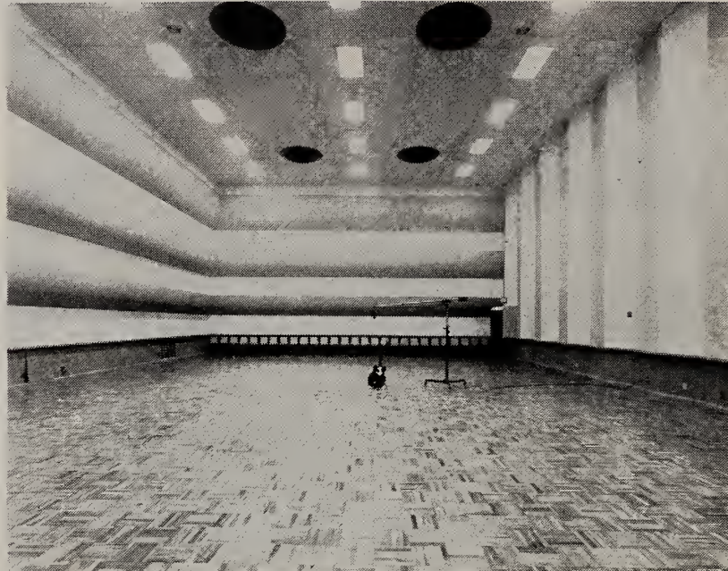
The modern new RCA Victor recording studio in Nashville is capable of com- fortably housing 100 performers in its 95,000 cubic feet. For perspective, the guitar was provided by Chet Atkins, operations manager, and recording star for Victor.
