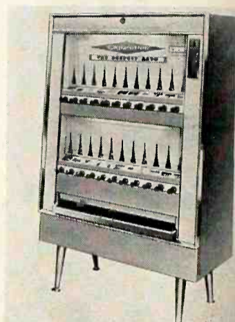
NATIONAL Crown Series 222; 22 cols.; 11 upper cols.; max. cap. 33; 11 lower max. cap. 23; total 616. Takes all sizes. Mechanical.
