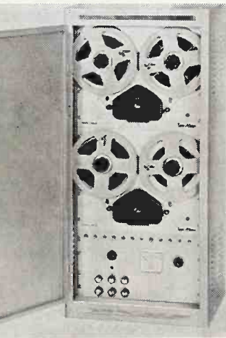
TAPE-ATHON LIBRARIAN Two tape transports (interconnected), 144 mode selective programming, automatic stand- by for continuous play, 12 activating toggle switches.
