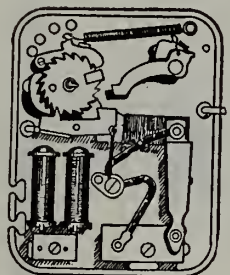
MAGAZINE SWITCH BOX ASSEMBLY
