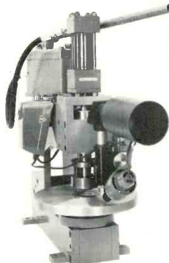
Stamper Centering Machine Model CMP-114
