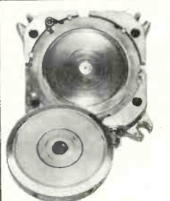
Alpha high speed moulds with interchangeable inserts
