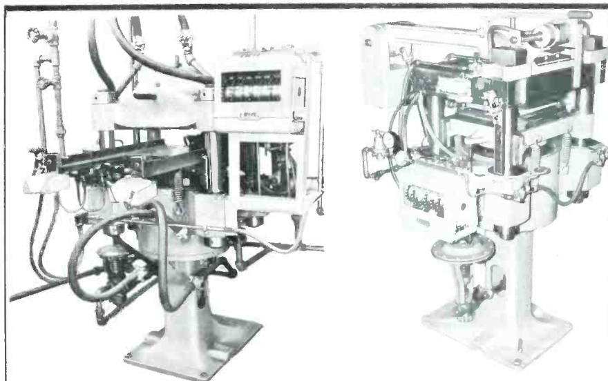
Model #BE-12" L.P. Record Press. Barnett 4-Post Press designed to handle book-type dies automatically.
