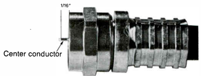
Figure 7: Center conductor trimming
