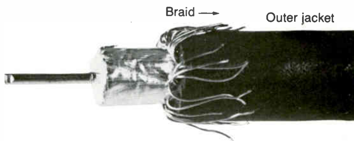
Figure 3: Braid folded over outer jacket
