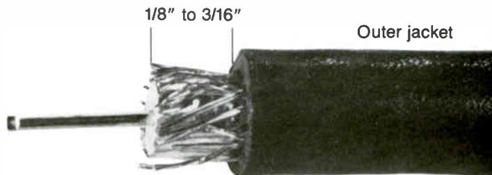
Figure 2: Outer jacket removal
