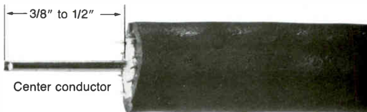
Figure 1: Center conductor exposure and cleaning
