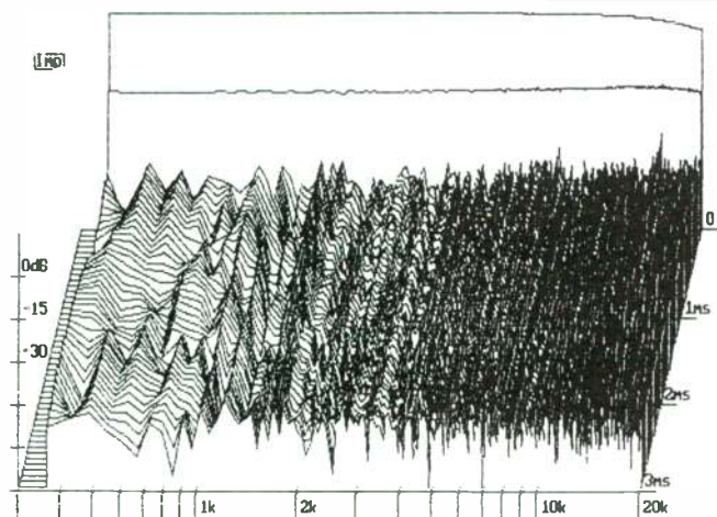
FIGURE 8: Waterfall plot of Cal signal, five averaged pulses.
