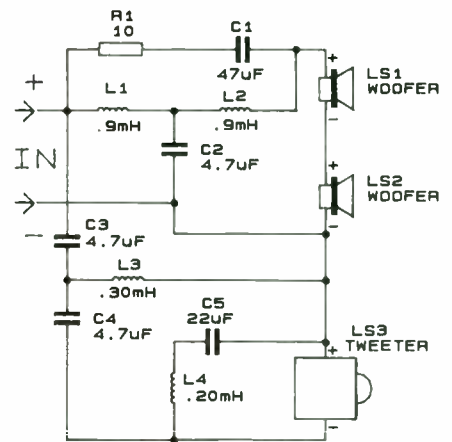
FIGURE 3: Crossover schematic/wiring diagram.
