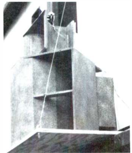
PHOTO 3: Detail of horn mounting.
