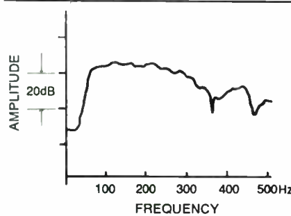
FIGURE 4: Response of 1984 design with diagonal reflectors.
