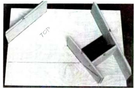
PHOTO 2: Throat partitions mounted to the top.
