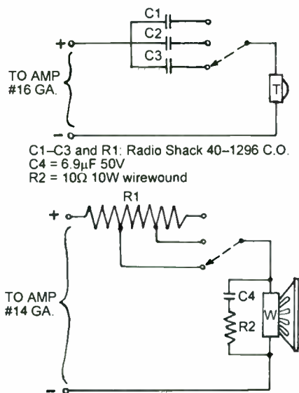
FIGURE 2: Biwired crossover for the Simplex speaker.
