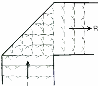
FIGURE 6: Huygen's wavefront construction for a 90° duct bend with a diagonal reflector. "I" is the incident wave; "R" is the reflected wave.
