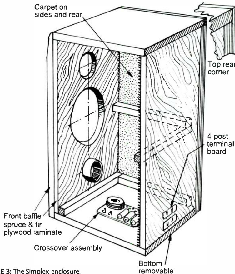
FIGURE 3: The Simplex enclosure.
