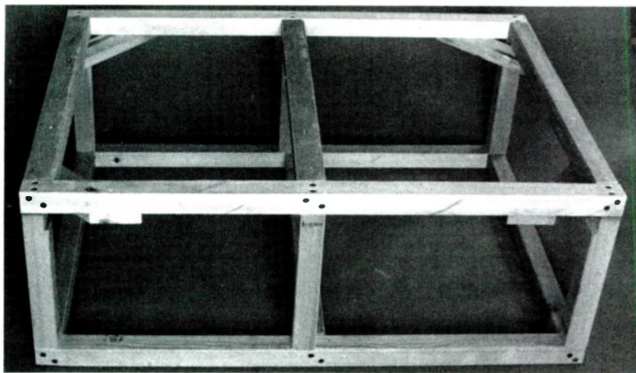
PHOTO 13: Finished 13½" stand.
