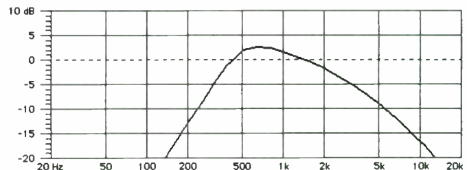
FIGURE 3: Sample custom filter response.
