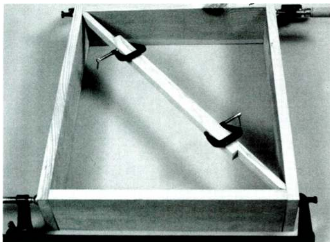
PHOTO 11: Checking the opposite diagonal.
