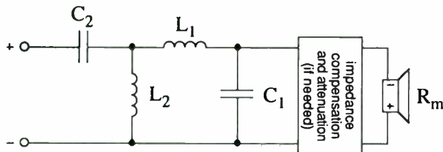
FIGURE 2: Second-order bandpass crossover.
