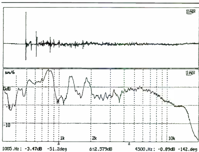
FIGURE 11: Pulse equivalent of Fig. 10. Note the quieter period just before the impulse.
