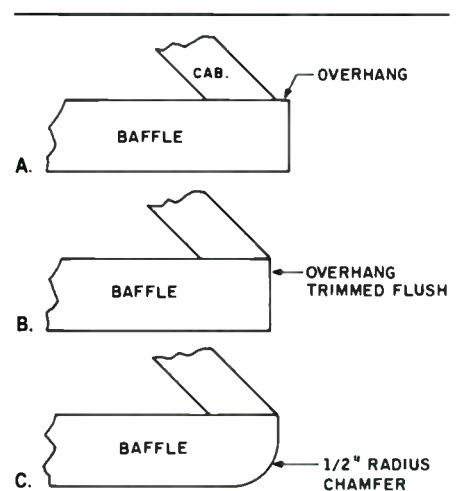
FIGURE 2: Baffle joint detail: a. with overhang; b. overhang trimmed flush; c. with chamfer.
