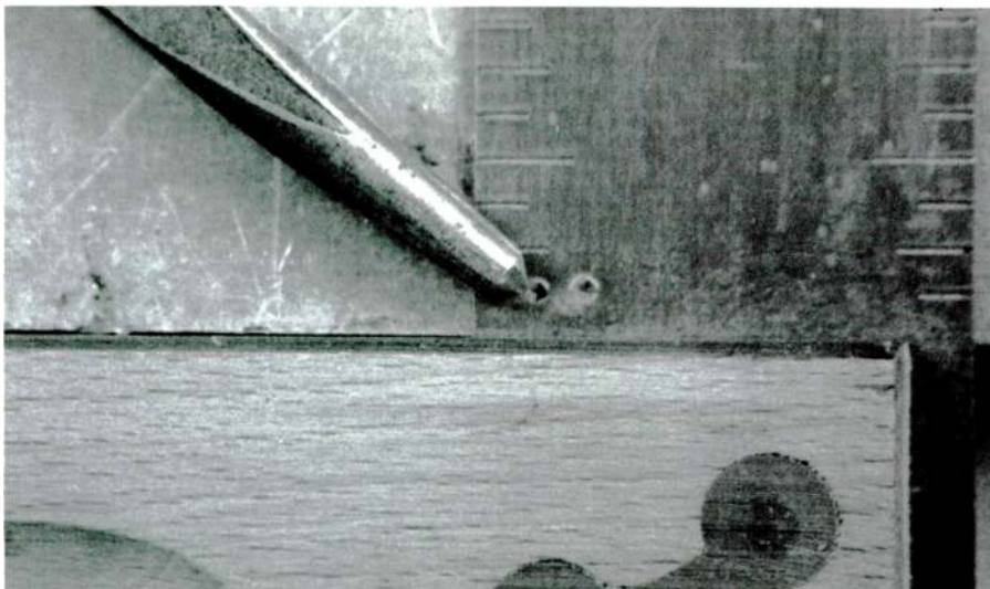
PHOTO 3: Peening the blade of the try square to obtain alignment.
