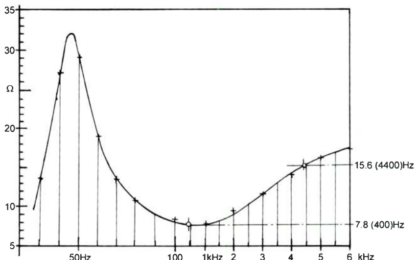
FIGURE 1: Impedance curve for the Radio Shack model 40-1011-A 6½" woofer.
