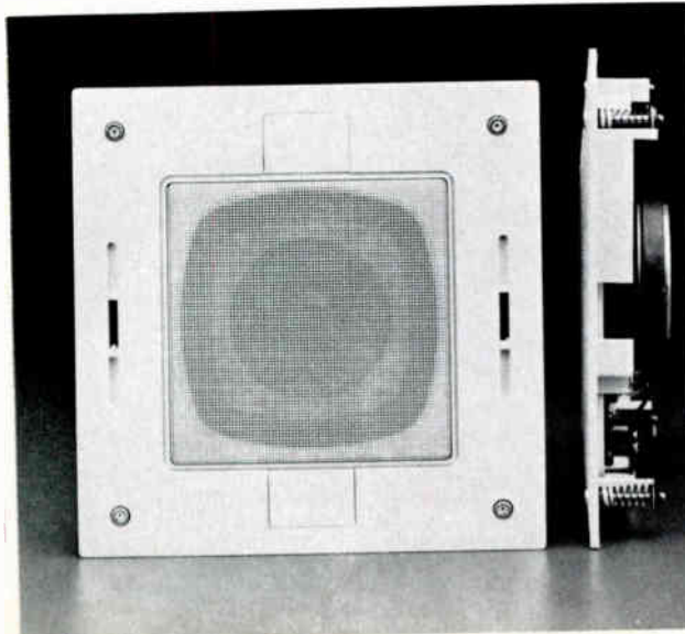
Spring-loaded bracket.
