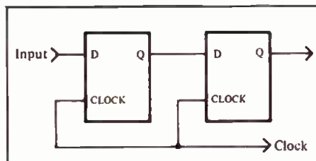
Figure 4. Double buffer.
