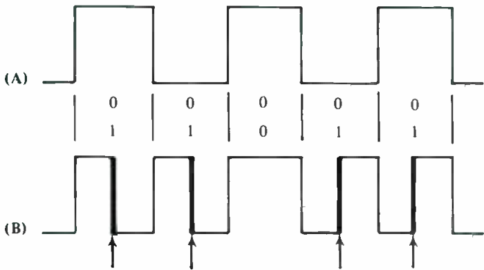
Figure 1. In the SMPTE time code, a zero is defined whenever there is no transition within a bit cell (A), while a transition within the bit cell (B) defines a one.
