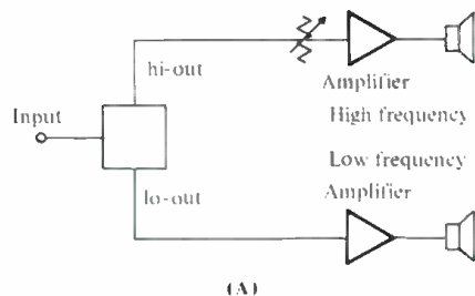
Figure 4. A More Robust Dividing Network for Sound Reinforcement.
