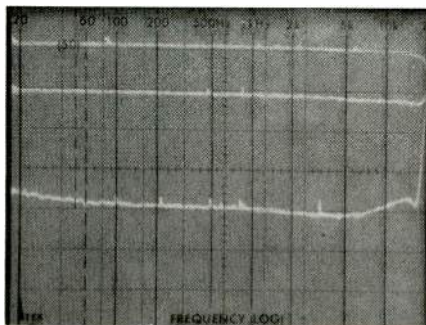
Fig. 3—Frequency response (top trace) and separation vs. frequency with blend activated (middle trace) and deactivated (bottom trace). Note flatness of middle trace (see text).
