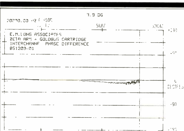
Fig. 7—Interchannel phase difference of arm/cartridge as a function of frequency (B & K 2011, band 7, pink noise). Phase difference at 20 kHz (cursor position) is 3.9°, equivalent to only 0.5 \mu S of interchannel delay.
