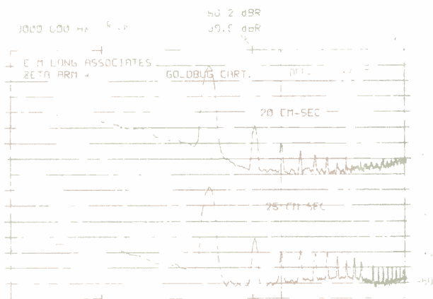
Fig. 9—Spectral analysis of the cartridge output when reproducing the test signal of Fig. 8. The third harmonic (at the cursor position) is 0.35% in the left channel and 1.05% in the right.
