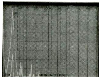
Fig. 4—Analysis of distortion and crosstalk for 5-kHz FM modulating frequency. Note lack of spurious crosstalk components and of subcarrier leakage.
