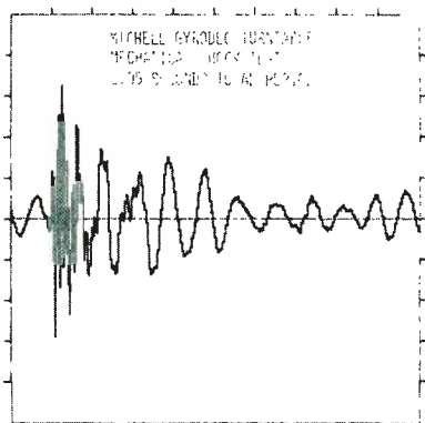
Fig. 7—Output vs. time response for mechanical shock applied to heavy platform on which the turntable rested. The GyroDec's isolation from the shock is excellent.
