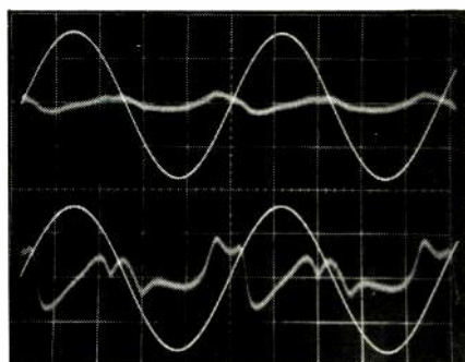
Fig. 6—Harmonic-distortion residue, 702 amp, for two frequencies, at 10 watts output into 8-ohm loads. Upper traces show 0.008% THD at 1 kHz; lower traces show 0.025% THD at 10 kHz. Note similarity between distortion waveforms (see text).
