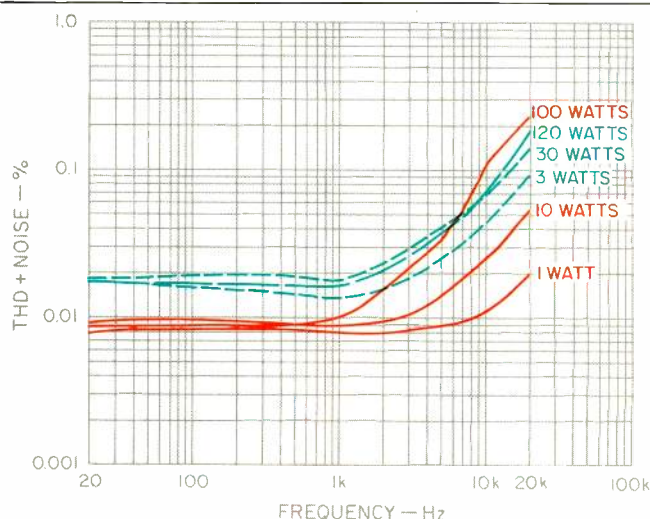
Fig. 5—THD + N vs. frequency, 702 amplifier, for power levels of 1, 10, and 100 watts into 8 ohms (solid curves) and 3, 30, and 120 watts into 4 ohms (dashed curves).
