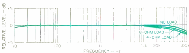
Fig. 8—Frequency response, 702 amp, with no load (open circuit) and with 8- and 4-ohm loads.
