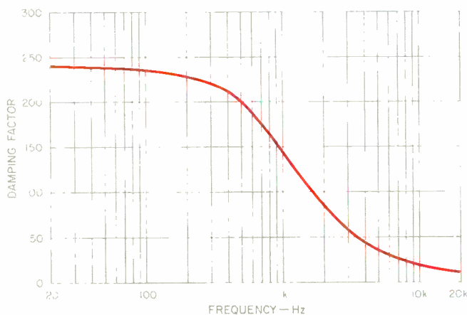
Fig. 10—Damping factor vs. frequency, right channel, 702 amp.
