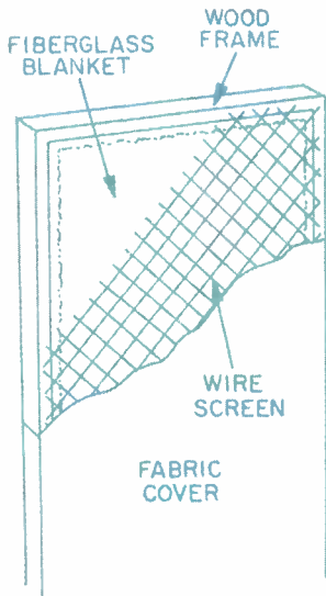
Fig. 3—Photo and cutaway view of absorption panel's construction. The panel should have a solid backing (not shown).
