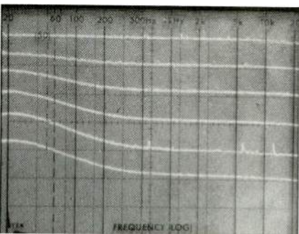
Fig. 7—Characteristics of loudness compensation. Note that only bass is affected.
