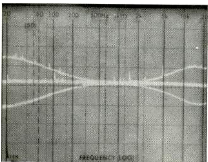
Fig. 6—Tone-control range, preamplifier section. Note absence of effect on midrange.
