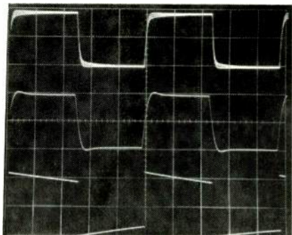
Fig. 9—Square-wave response, 702 amp. Top traces: 10 kHz into 8- and 4-ohm resistive loads and into open circuit (no load). Middle trace: 10 kHz into 8 ohm, 2- \mu F load. Bottom trace: 40 Hz into 8-ohm load. Scales: Vertical, 5 V/div.; horizontal, 20 \mu s/div. for 10-kHz traces, 5 ms/div. for 40-Hz trace.
