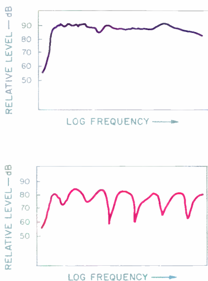
Fig. 2—Frequency response of reference loudspeaker system under anechoic conditions (A) and with effects of early reflections (about 1.1 mS delay) added (B). (After Davis.)
