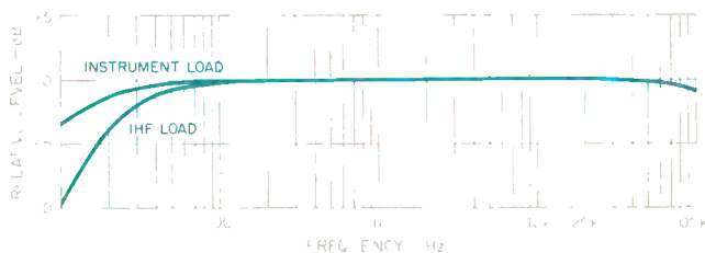
Fig. 1—Line-level frequency response, 402 preamplifier, for reviewer's instrument load (see text) and for standard IHF load.
