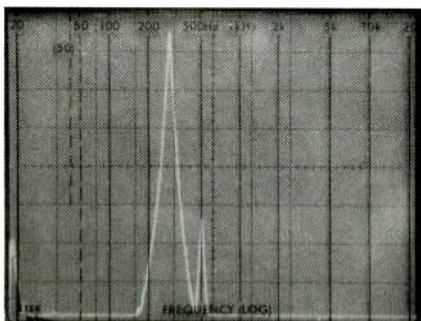
Fig. 4—Spectrum analysis of reproduced 20-kHz test signal. Note the lack of in-band beat components.
