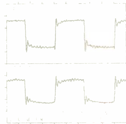
Fig. 12—Output from 1-kHz square wave, CBS STR-112 test record. Ringing is at 27.8 kHz.
