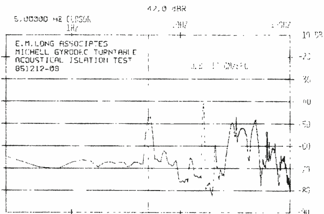
Fig. 9—Spectrum (to 100 Hz) of the vibrations from a 100 dB SPL acoustic field at the surface of a record. Cartridge stylus is resting in a groove near the middle of the record.
