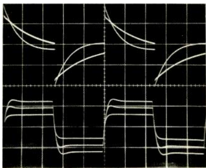
Fig. 2—Square-wave response, 402 preamp line-amplifier section. Upper traces are for 20-Hz signal, with instrument load and (showing greater tilt) with IHF load. Lower traces are for 20 kHz, right channel, with balance control set full right (largest trace), centered, and set full left (smallest trace). Scales: Vertical, 2 V/div.; horizontal, 10 mS/div. (upper traces), 10 \mu S/div. (lower traces).
