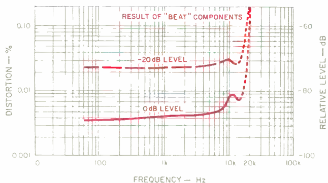
Fig. 3—THD vs. frequency, at two output levels (see text).
