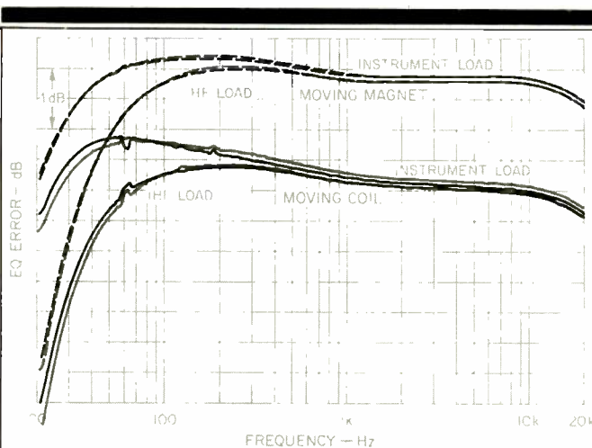
Fig. 3—RIAA equalization error for 402 preamp's MM and MC inputs, with instrument and IHF loads. Note the low-end roll-off and the expanded scale.
