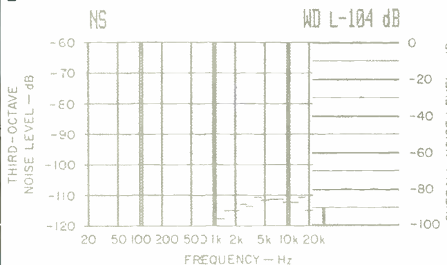
Fig. 2—S/N analysis, both unweighted (A) and A-weighted (B).
