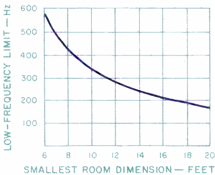
Fig. 4—Lowest effective frequency for acoustic-panel absorbers as a function of room size (where f = 3,390/\text{smallest room dimension in feet} ). For frequencies below those shown, other forms of absorption (such as wave cavities) would be needed.
