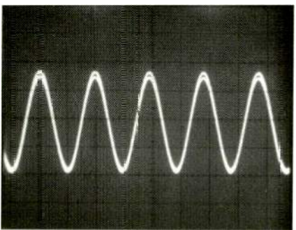
Fig. 8—Interchannel phase difference when reproducing a 20-kHz tone. One trace was vertically displaced for clarity.
