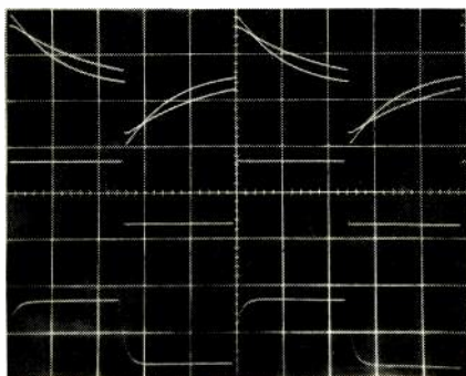
Fig. 4—MM phono response, 402 preamp, to pre-equalized square waves at 40 Hz (top traces), 1 kHz (middle trace), and 10 kHz (bottom trace). Note effects of IHF (greater tilt) and instrument loads at 40 Hz. Scales: Vertical, 2 V/div.; horizontal, 5 mS/div. (top), 200 \mu S/div. (middle), 20 \mu S/div. (bottom).
