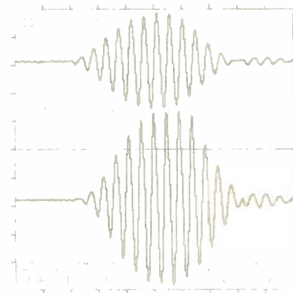
Fig. 10—Output from 15- and 30-cm/S, 10.8-kHz pulse test, Shure TTR-103 test record. Note the small amount of asymmetry and compression.
