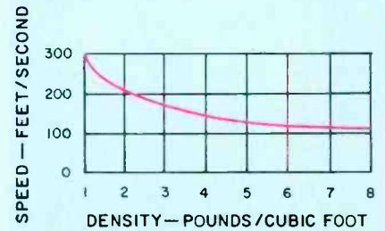
Fig. B1—Speed of sound versus packing density of material. Speed in air is normally 1,130 feet per second. (After Bradbury.)
