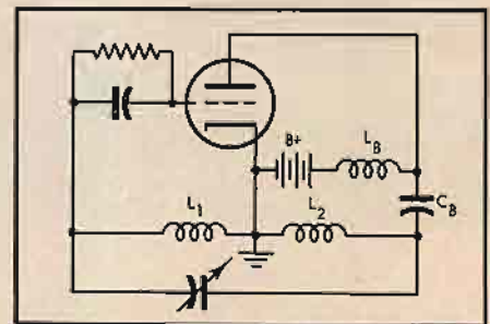
Fig. 2. Hartley oscillator.
