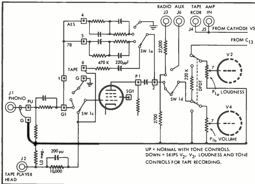
Fig. 6. Schematic of modifications to one of the preamps to permit direct connection from tape head as well as to eliminate tone and loudness controls from the circuit for recording.
