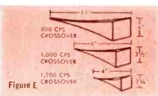
Figure E shows representative horns, illustrating that horns must have a certain length, as well as cross sectional area along their length and at the mouth to load the driver diaphragm down to the lowest frequencies to be reproduced. The lower we go, the longer must be the horn and the greater the mouth area.
