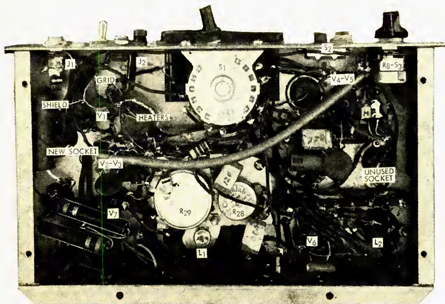
Fig. 3. Underchassis view of the completed amplifier.
