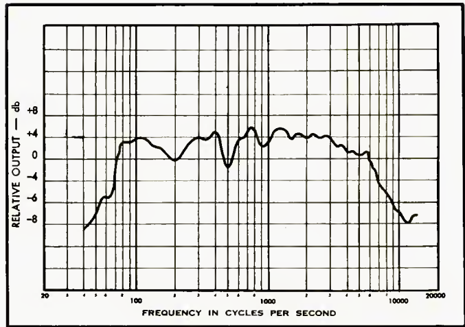
Fig. 4. Unequalized response measurement of the complete system.
