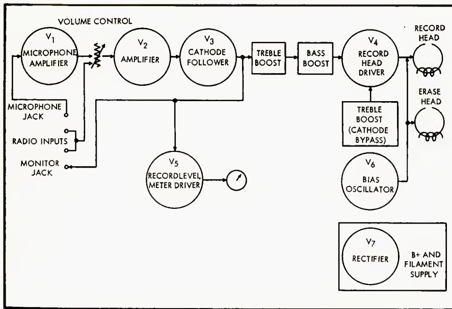
Fig. 5. Functions of the amplifier in the record mode.
