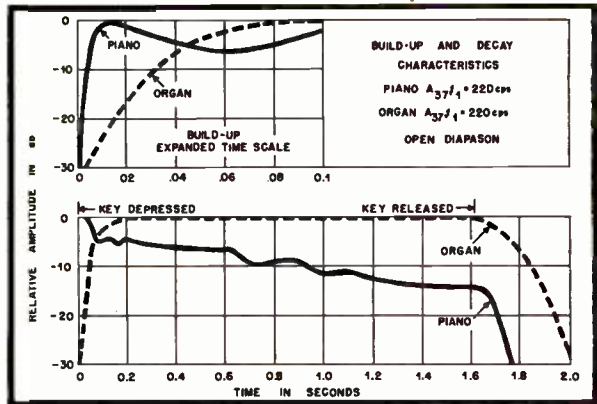
Fig. 17. Build-up and decay characteristics of organ and piano tones.
