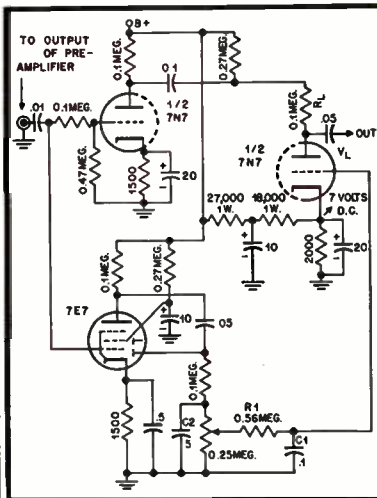
Fig. 14—14. Variable-plate-resistance volume expander. The attack time, in seconds, is the time constant ( R \times C ) of R_1 and C_1 , and the release time is the time constant of the potentiometer and C_2 plus R_2 . The potentiometer controls the amount of expansion, to a maximum of about 7 db. (After McProud.)
