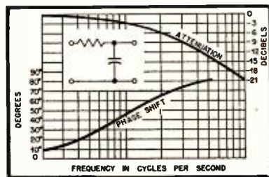
Fig. 14-6. Phase shift in relation to attenuation of an R-C network. (After F. Langford Smith.)
